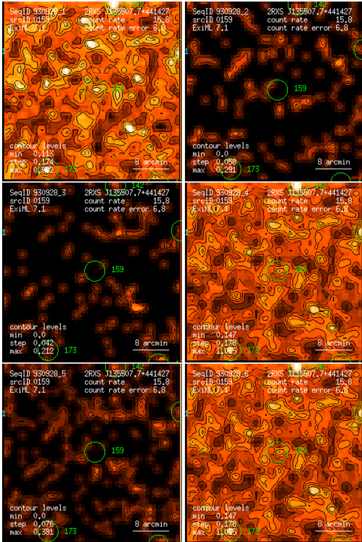
Figure 159: RASS 930928: detection 0159: band rate images, Gaussian filter: (1) PSPC channels 11 – 41, (2) 52 – 90, (3) 91 – 201, (4) 11 – 235, (5) 52 – 201, (6) 11 – 201. Broad band rates in counts/ks. Band rate contour levels in counts/ks/arcmin 2 .
