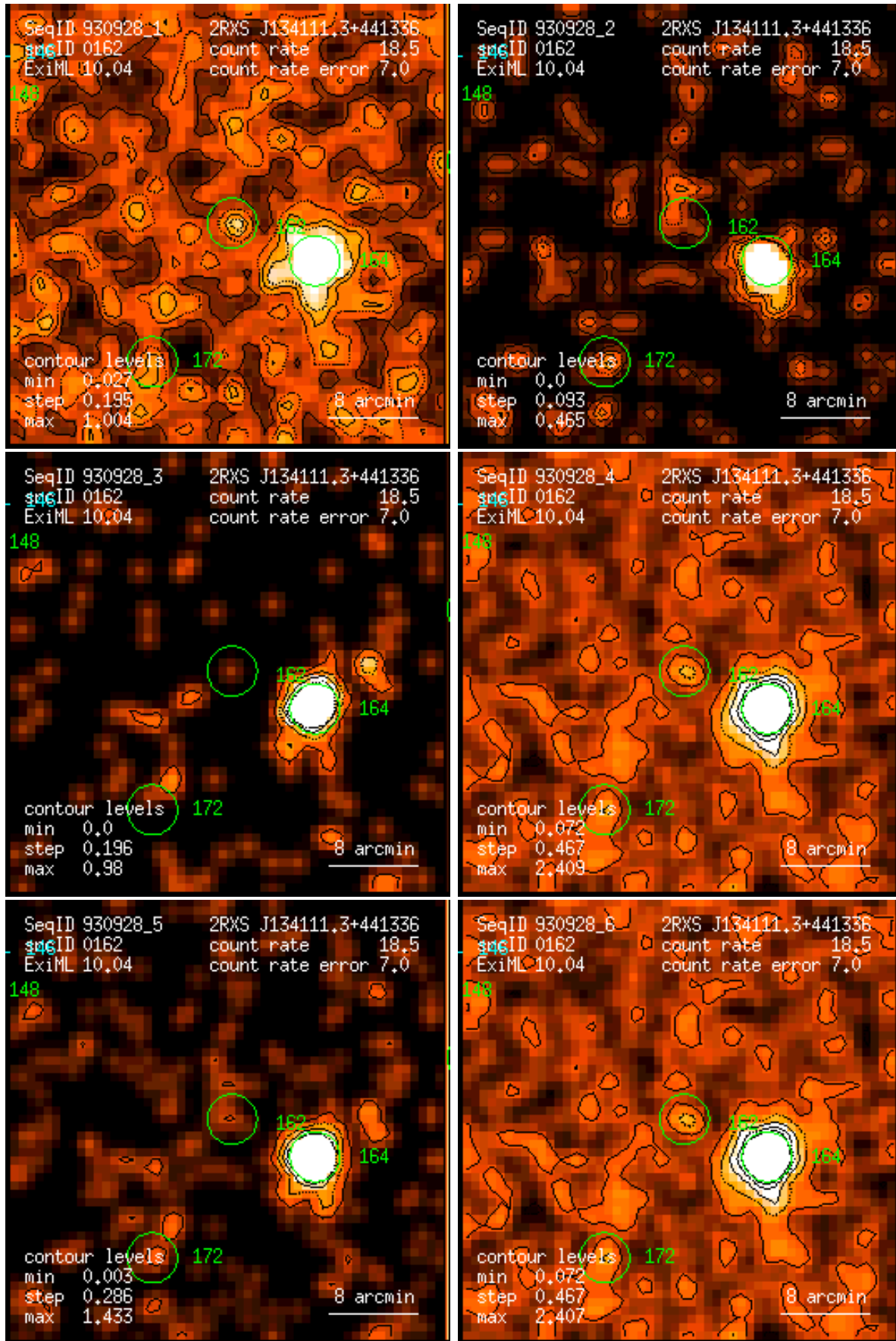
Figure 162: RASS 930928: detection 0162: band rate images, Gaussian filter: (1) PSPC channels 11 – 41, (2) 52 – 90, (3) 91 – 201, (4) 11 – 235, (5) 52 – 201, (6) 11 – 201. Broad band rates in counts/ks. Band rate contour levels in counts/ks/arcmin 2 .
