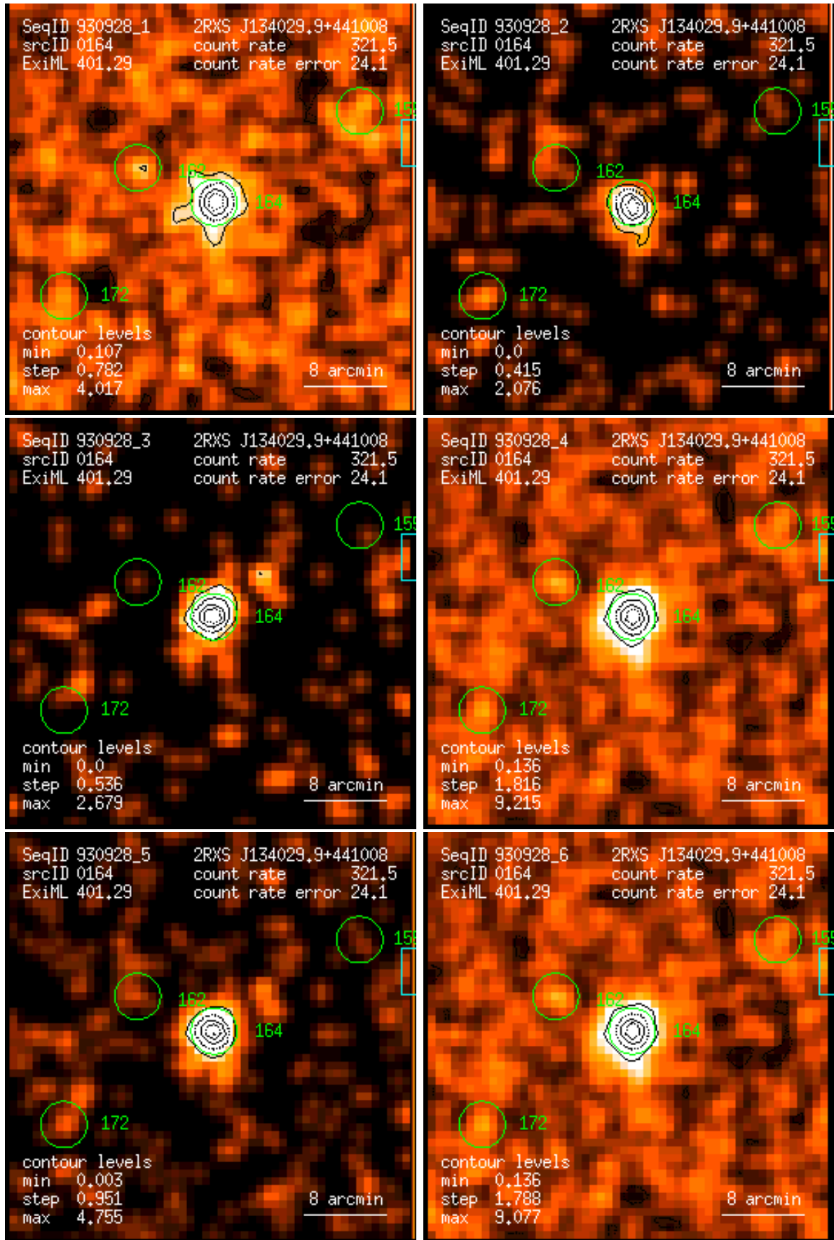
Figure 164: RASS 930928: detection 0164: band rate images, Gaussian filter: (1) PSPC channels 11 – 41, (2) 52 – 90, (3) 91 – 201, (4) 11 – 235, (5) 52 – 201, (6) 11 – 201. Broad band rates in counts/ks. Band rate contour levels in counts/ks/arcmin 2 .
