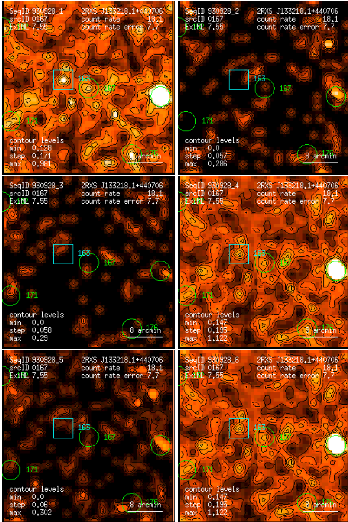
Figure 167: RASS 930928: detection 0167: band rate images, Gaussian filter: (1) PSPC channels 11 – 41, (2) 52 – 90, (3) 91 – 201, (4) 11 – 235, (5) 52 – 201, (6) 11 – 201. Broad band rates in counts/ks. Band rate contour levels in counts/ks/arcmin 2 .
