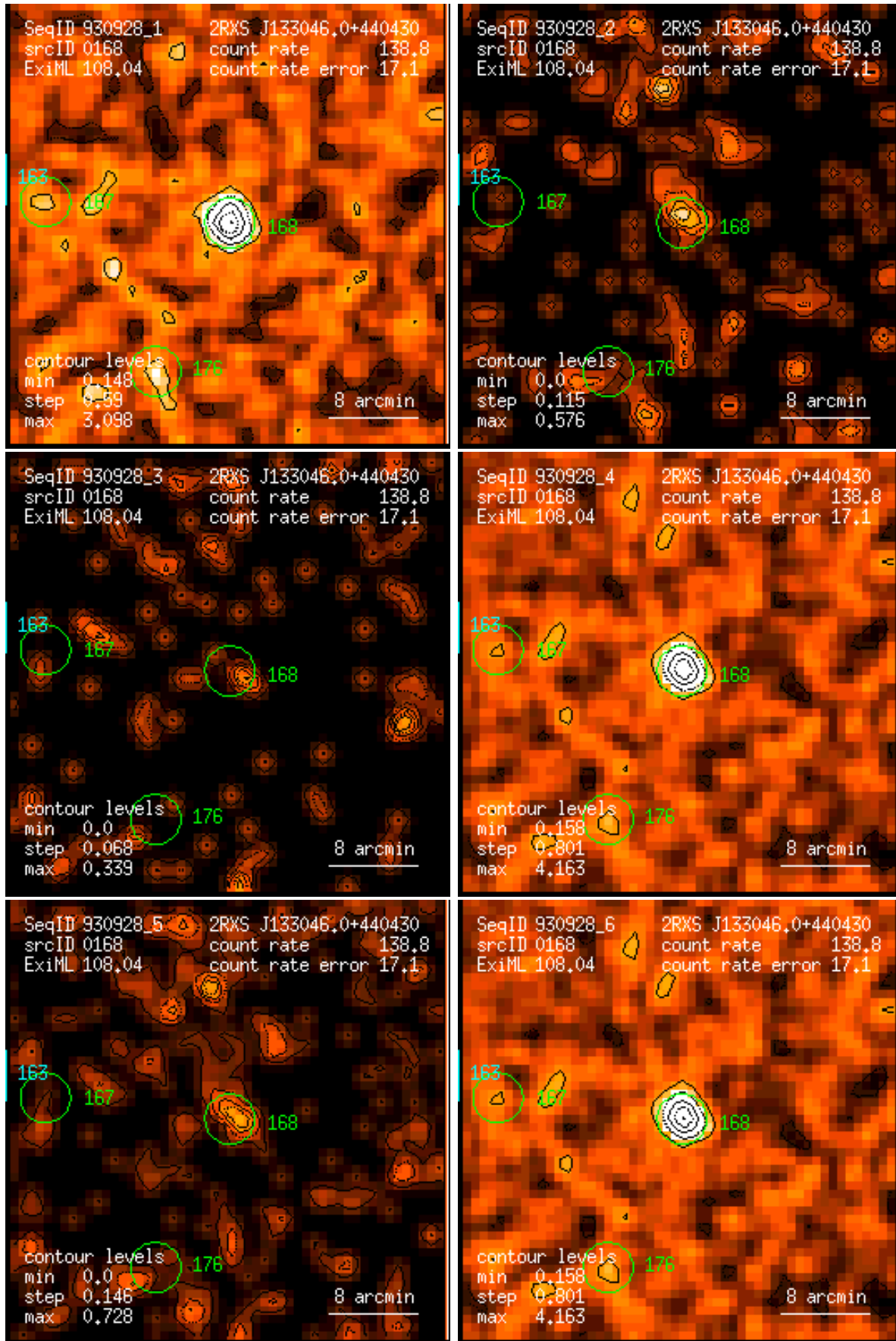
Figure 168: RASS 930928: detection 0168: band rate images, Gaussian filter: (1) PSPC channels 11 – 41, (2) 52 – 90, (3) 91 – 201, (4) 11 – 235, (5) 52 – 201, (6) 11 – 201. Broad band rates in counts/ks. Band rate contour levels in counts/ks/arcmin 2 .
