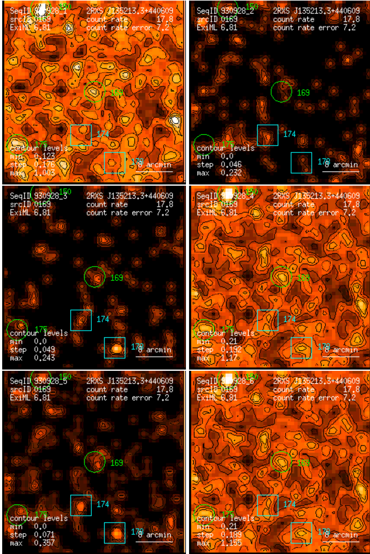
Figure 169: RASS 930928: detection 0169: band rate images, Gaussian filter: (1) PSPC channels 11 – 41, (2) 52 – 90, (3) 91 – 201, (4) 11 – 235, (5) 52 – 201, (6) 11 – 201. Broad band rates in counts/ks. Band rate contour levels in counts/ks/arcmin 2 .
