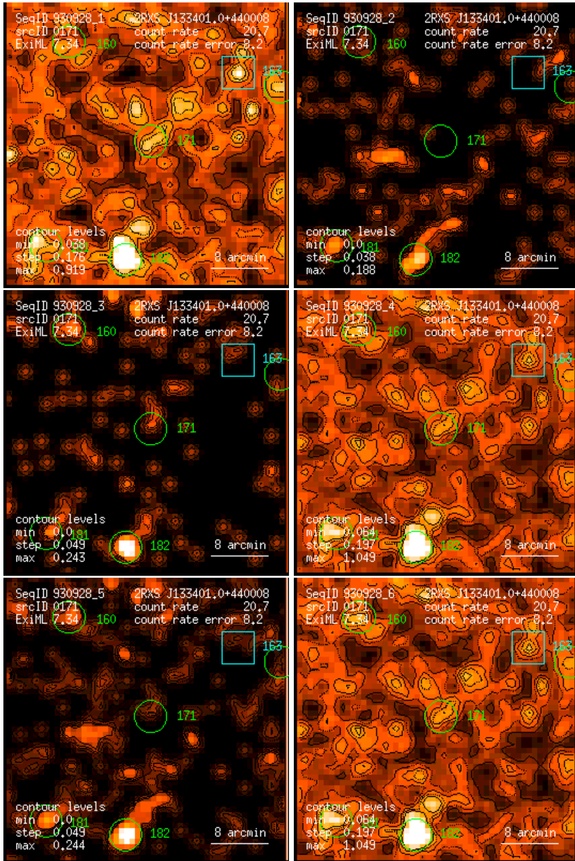
Figure 171: RASS 930928: detection 0171: band rate images, Gaussian filter: (1) PSPC channels 11 – 41, (2) 52 – 90, (3) 91 – 201, (4) 11 – 235, (5) 52 – 201, (6) 11 – 201. Broad band rates in counts/ks. Band rate contour levels in counts/ks/arcmin 2 .
