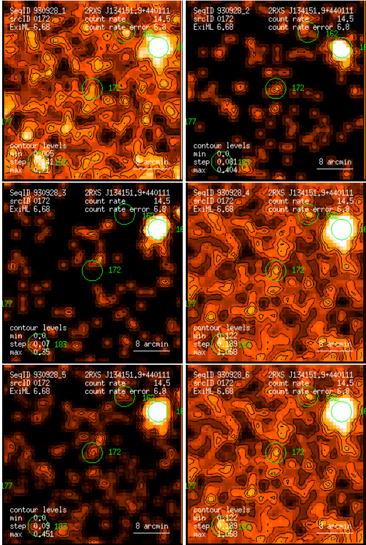
Figure 172: RASS 930928: detection 0172: band rate images, Gaussian filter: (1) PSPC channels 11 – 41, (2) 52 – 90, (3) 91 – 201, (4) 11 – 235, (5) 52 – 201, (6) 11 – 201. Broad band rates in counts/ks. Band rate contour levels in counts/ks/arcmin 2 .
