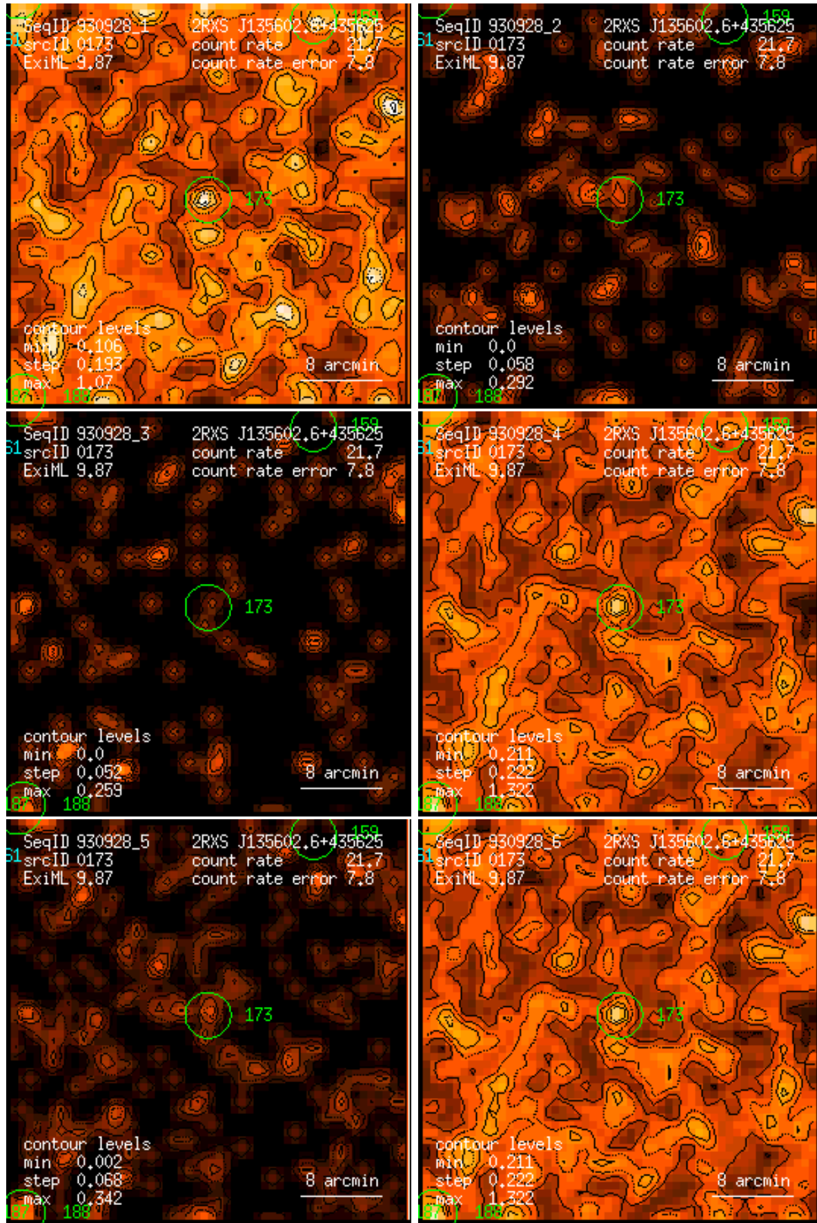
Figure 173: RASS 930928: detection 0173: band rate images, Gaussian filter: (1) PSPC channels 11 – 41, (2) 52 – 90, (3) 91 – 201, (4) 11 – 235, (5) 52 – 201, (6) 11 – 201. Broad band rates in counts/ks. Band rate contour levels in counts/ks/arcmin 2 .
