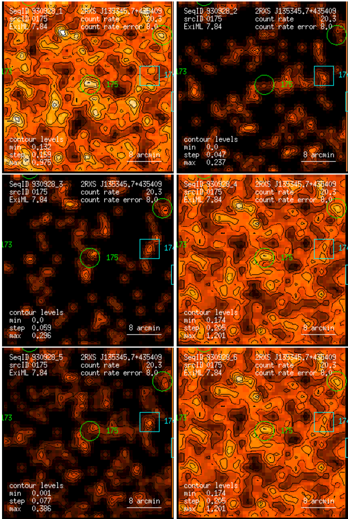
Figure 175: RASS 930928: detection 0175: band rate images, Gaussian filter: (1) PSPC channels 11 – 41, (2) 52 – 90, (3) 91 – 201, (4) 11 – 235, (5) 52 – 201, (6) 11 – 201. Broad band rates in counts/ks. Band rate contour levels in counts/ks/arcmin 2 .
