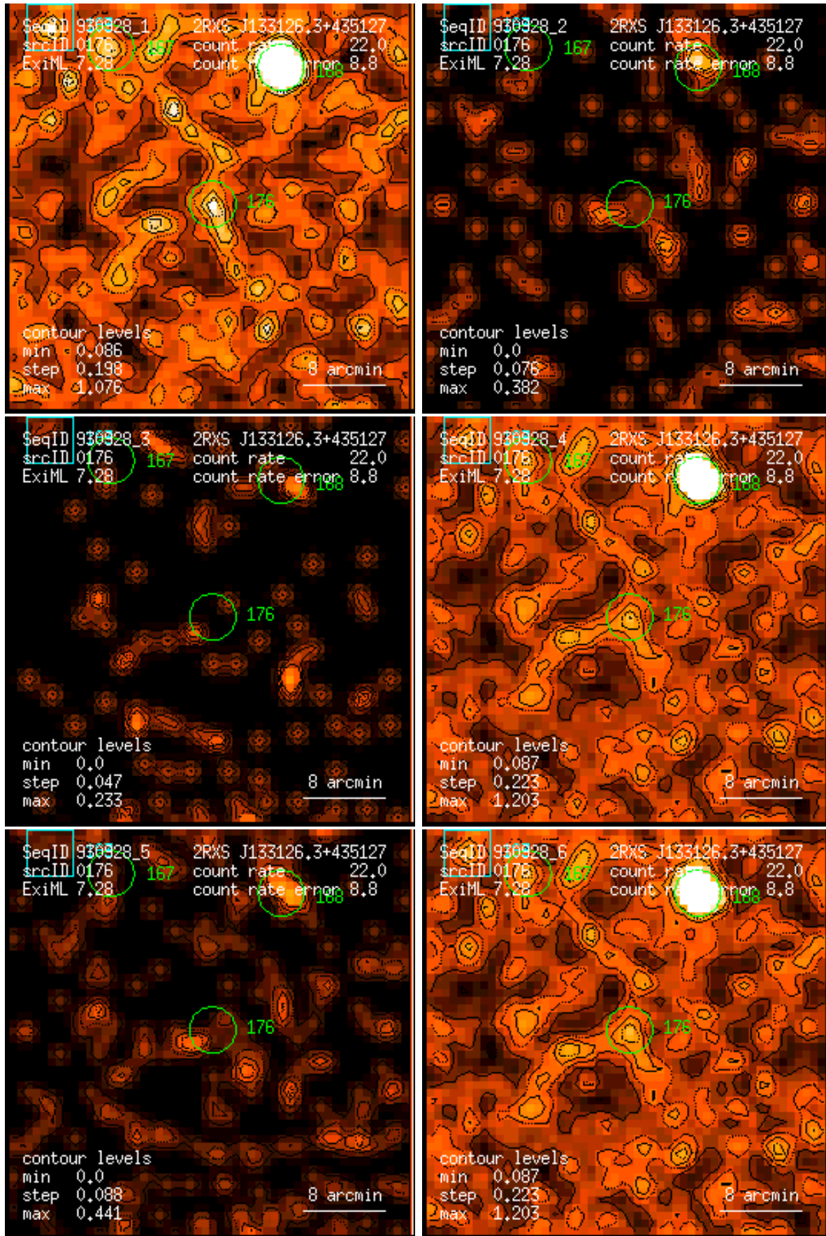
Figure 176: RASS 930928: detection 0176: band rate images, Gaussian filter: (1) PSPC channels 11 – 41, (2) 52 – 90, (3) 91 – 201, (4) 11 – 235, (5) 52 – 201, (6) 11 – 201. Broad band rates in counts/ks. Band rate contour levels in counts/ks/arcmin 2 .
