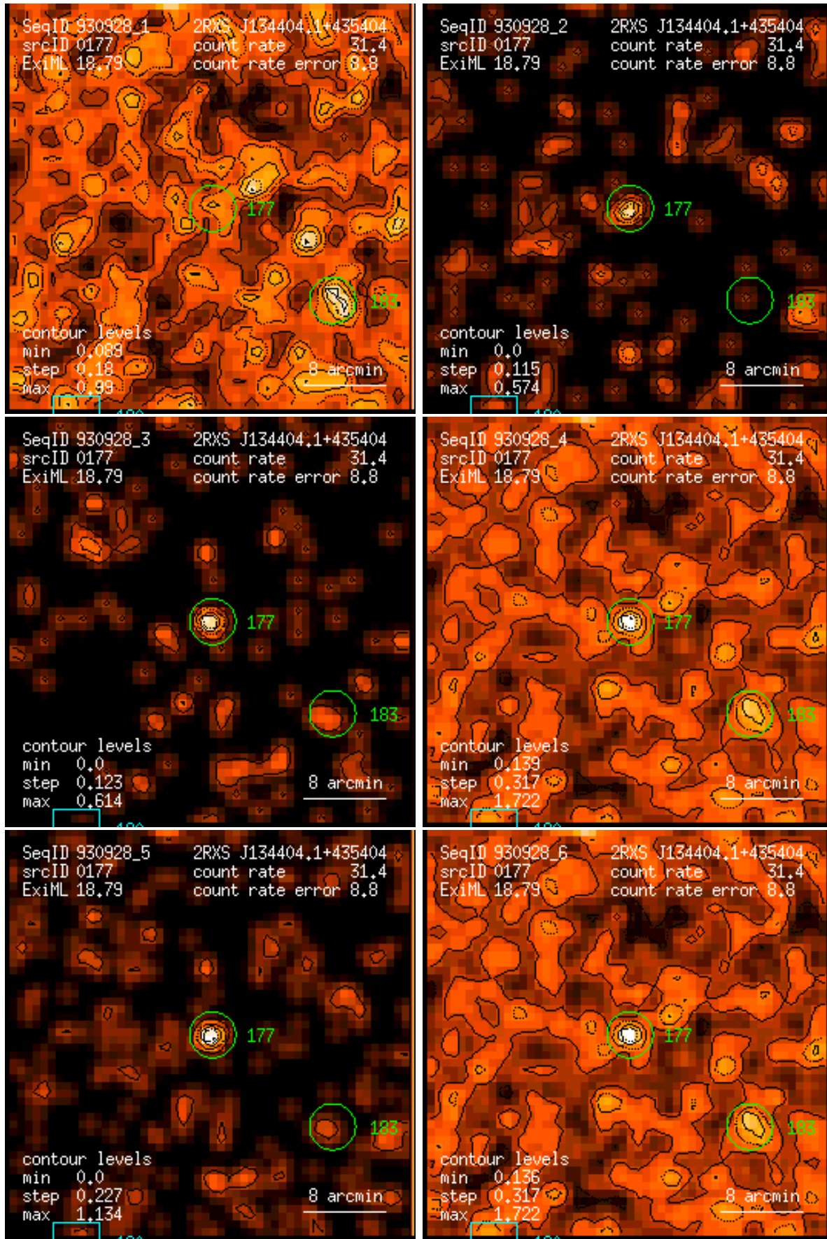
Figure 177: RASS 930928: detection 0177: band rate images, Gaussian filter: (1) PSPC channels 11 – 41, (2) 52 – 90, (3) 91 – 201, (4) 11 – 235, (5) 52 – 201, (6) 11 – 201. Broad band rates in counts/ks. Band rate contour levels in counts/ks/arcmin 2 .
