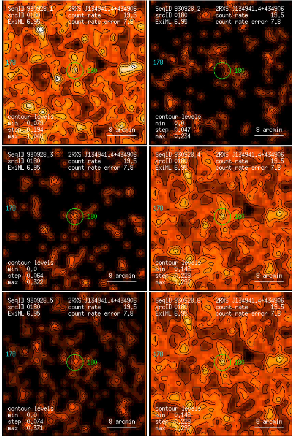
Figure 180: RASS 930928: detection 0180: band rate images, Gaussian filter: (1) PSPC channels 11 – 41, (2) 52 – 90, (3) 91 – 201, (4) 11 – 235, (5) 52 – 201, (6) 11 – 201. Broad band rates in counts/ks. Band rate contour levels in counts/ks/arcmin 2 .
