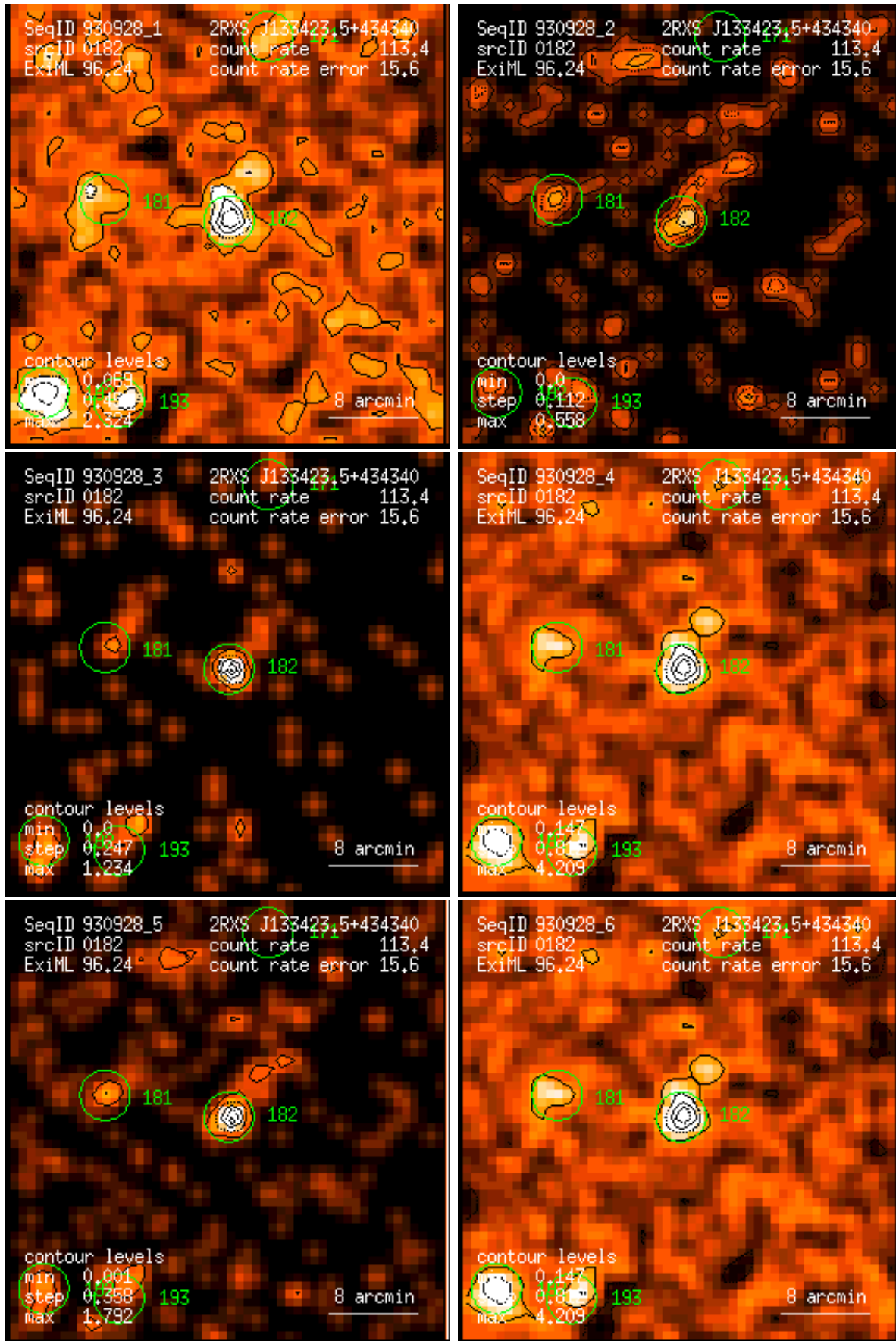
Figure 182: RASS 930928: detection 0182: band rate images, Gaussian filter: (1) PSPC channels 11 – 41, (2) 52 – 90, (3) 91 – 201, (4) 11 – 235, (5) 52 – 201, (6) 11 – 201. Broad band rates in counts/ks. Band rate contour levels in counts/ks/arcmin 2 .
