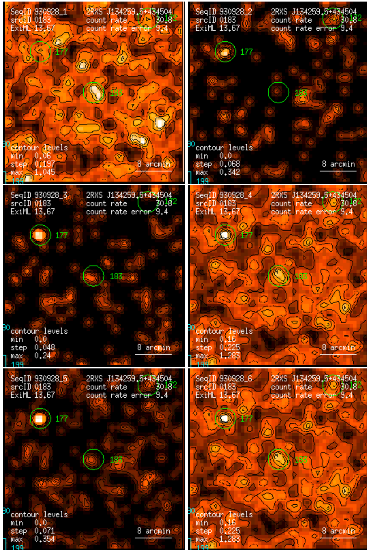
Figure 183: RASS 930928: detection 0183: band rate images, Gaussian filter: (1) PSPC channels 11 – 41, (2) 52 – 90, (3) 91 – 201, (4) 11 – 235, (5) 52 – 201, (6) 11 – 201. Broad band rates in counts/ks. Band rate contour levels in counts/ks/arcmin 2 .
