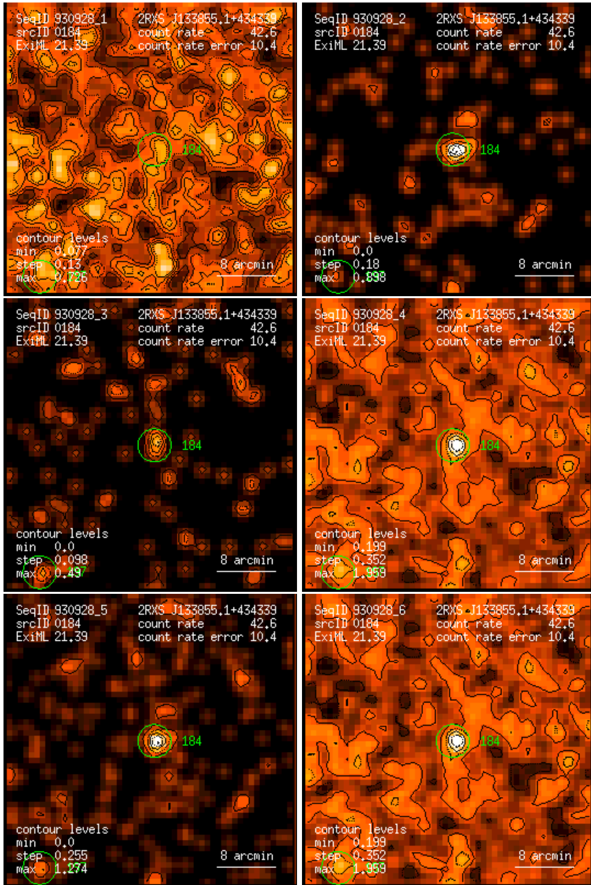
Figure 184: RASS 930928: detection 0184: band rate images, Gaussian filter: (1) PSPC channels 11 – 41, (2) 52 – 90, (3) 91 – 201, (4) 11 – 235, (5) 52 – 201, (6) 11 – 201. Broad band rates in counts/ks. Band rate contour levels in counts/ks/arcmin 2 .
