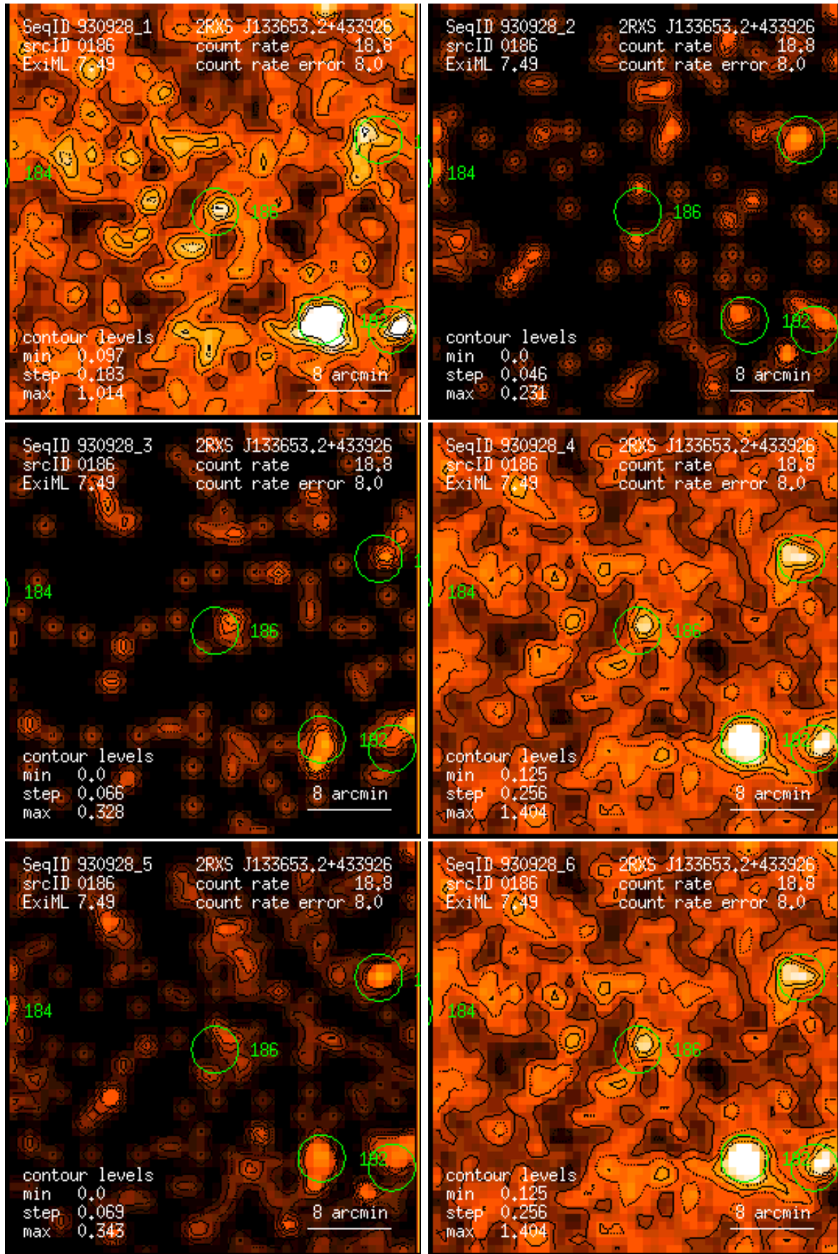
Figure 186: RASS 930928: detection 0186: band rate images, Gaussian filter: (1) PSPC channels 11 – 41, (2) 52 – 90, (3) 91 – 201, (4) 11 – 235, (5) 52 – 201, (6) 11 – 201. Broad band rates in counts/ks. Band rate contour levels in counts/ks/arcmin 2 .
