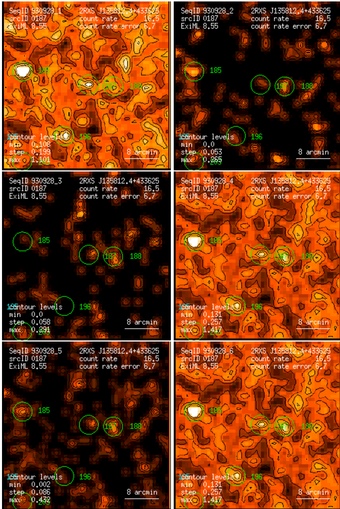
Figure 187: RASS 930928: detection 0187: band rate images, Gaussian filter: (1) PSPC channels 11 – 41, (2) 52 – 90, (3) 91 – 201, (4) 11 – 235, (5) 52 – 201, (6) 11 – 201. Broad band rates in counts/ks. Band rate contour levels in counts/ks/arcmin 2 .
