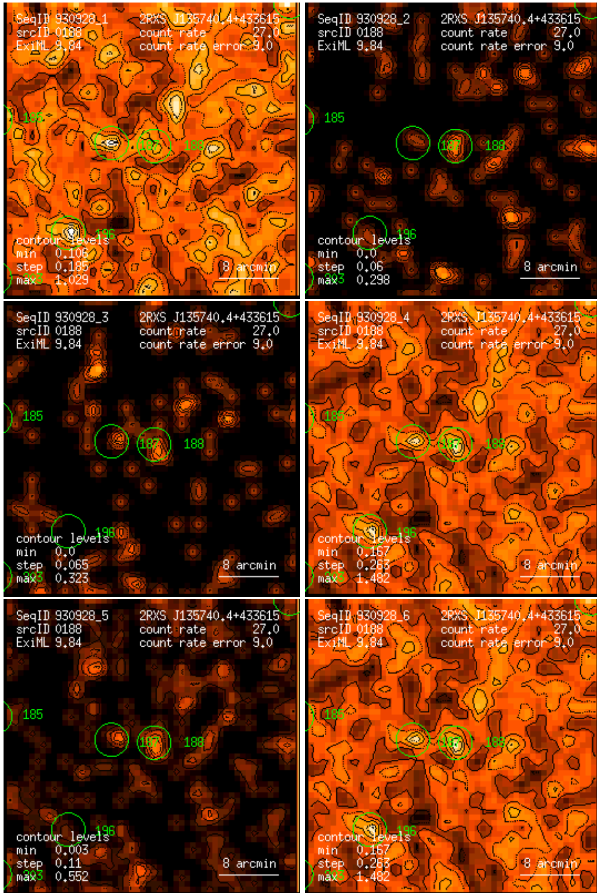
Figure 188: RASS 930928: detection 0188: band rate images, Gaussian filter: (1) PSPC channels 11 – 41, (2) 52 – 90, (3) 91 – 201, (4) 11 – 235, (5) 52 – 201, (6) 11 – 201. Broad band rates in counts/ks. Band rate contour levels in counts/ks/arcmin 2 .
