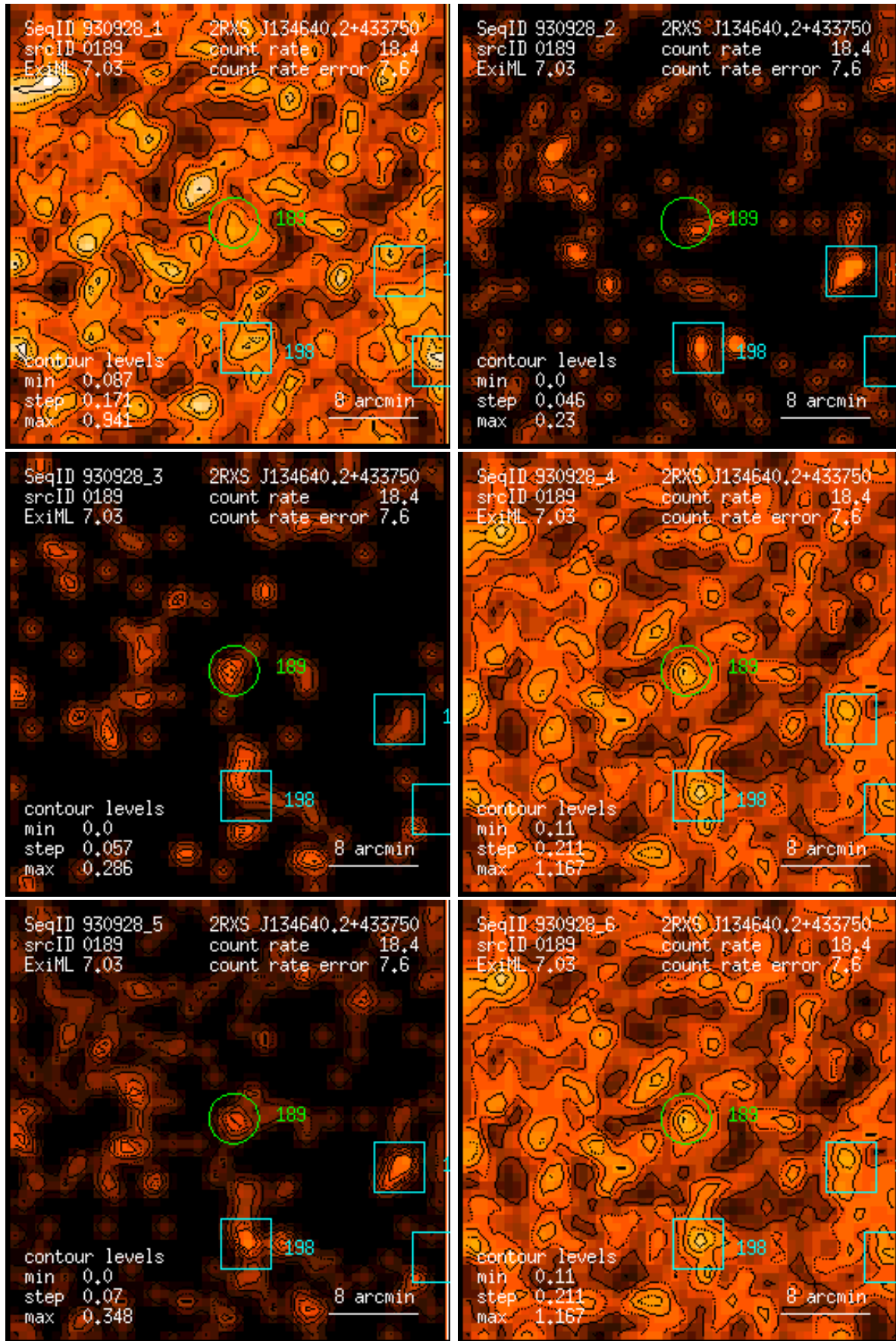
Figure 189: RASS 930928: detection 0189: band rate images, Gaussian filter: (1) PSPC channels 11 – 41, (2) 52 – 90, (3) 91 – 201, (4) 11 – 235, (5) 52 – 201, (6) 11 – 201. Broad band rates in counts/ks. Band rate contour levels in counts/ks/arcmin 2 .
