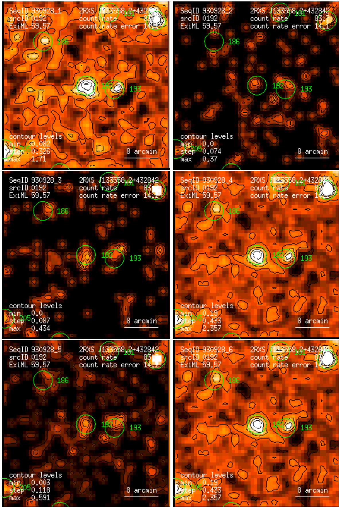
Figure 192: RASS 930928: detection 0192: band rate images, Gaussian filter: (1) PSPC channels 11 – 41, (2) 52 – 90, (3) 91 – 201, (4) 11 – 235, (5) 52 – 201, (6) 11 – 201. Broad band rates in counts/ks. Band rate contour levels in counts/ks/arcmin 2 .
