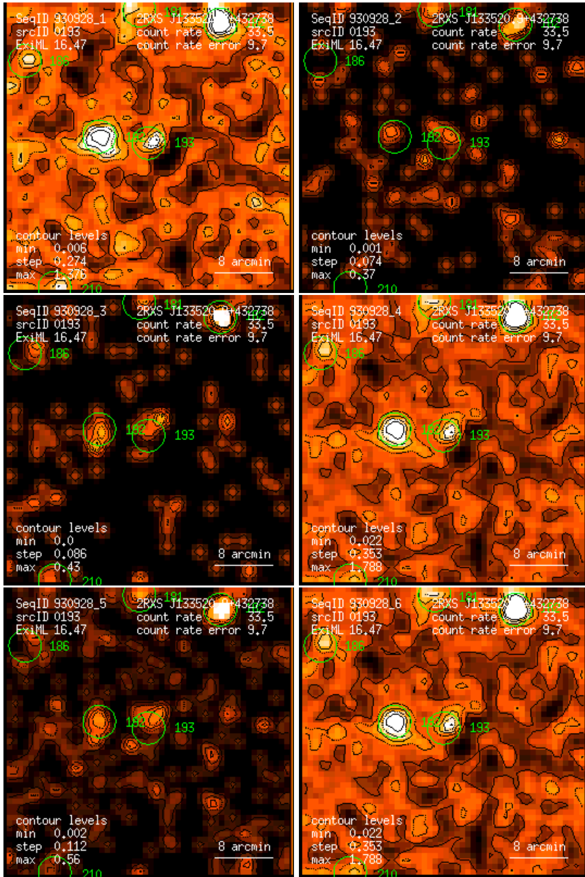
Figure 193: RASS 930928: detection 0193: band rate images, Gaussian filter: (1) PSPC channels 11 – 41, (2) 52 – 90, (3) 91 – 201, (4) 11 – 235, (5) 52 – 201, (6) 11 – 201. Broad band rates in counts/ks. Band rate contour levels in counts/ks/arcmin 2 .
