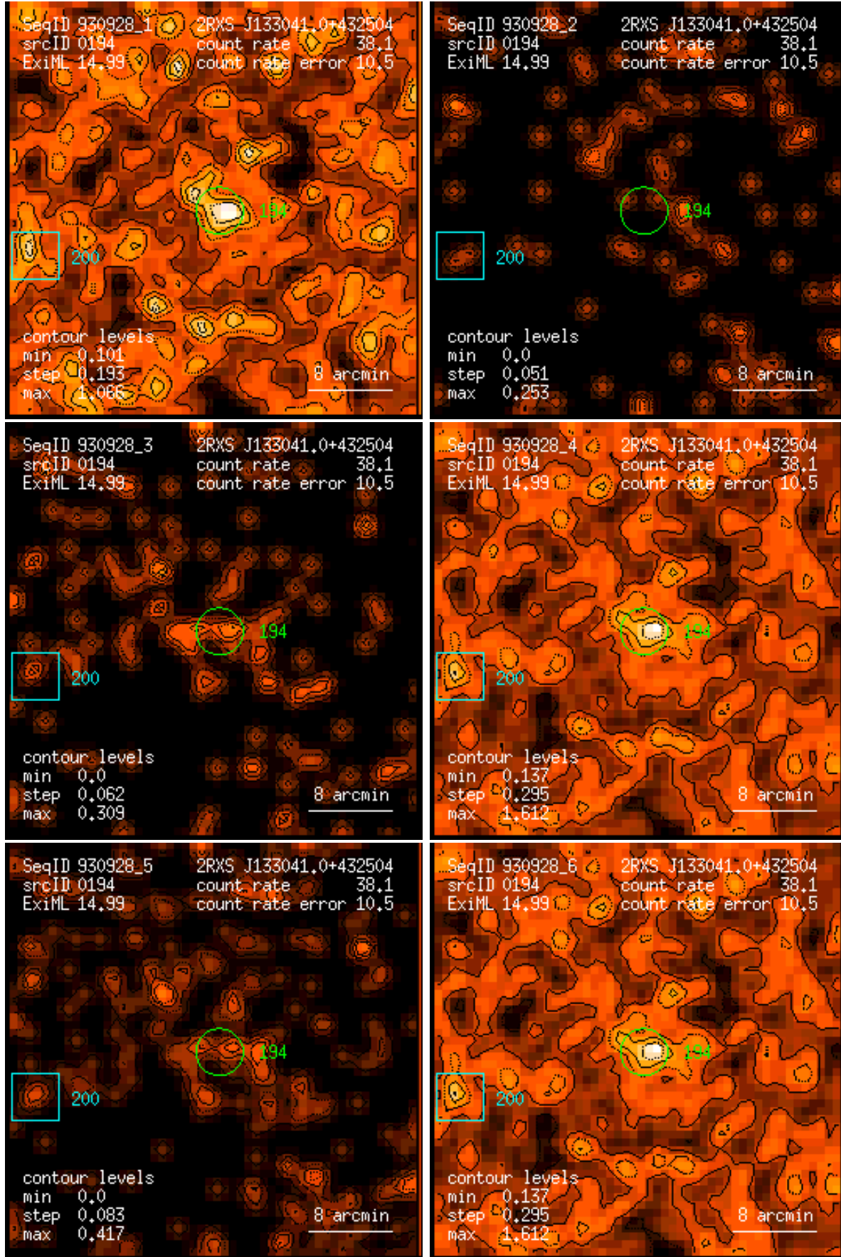
Figure 194: RASS 930928: detection 0194: band rate images, Gaussian filter: (1) PSPC channels 11 – 41, (2) 52 – 90, (3) 91 – 201, (4) 11 – 235, (5) 52 – 201, (6) 11 – 201. Broad band rates in counts/ks. Band rate contour levels in counts/ks/arcmin 2 .
