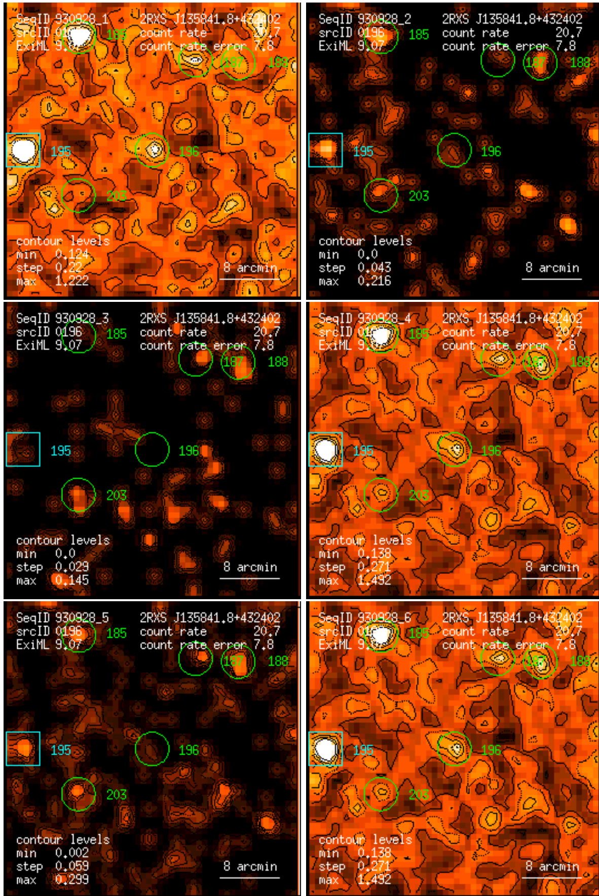
Figure 196: RASS 930928: detection 0196: band rate images, Gaussian filter: (1) PSPC channels 11 – 41, (2) 52 – 90, (3) 91 – 201, (4) 11 – 235, (5) 52 – 201, (6) 11 – 201. Broad band rates in counts/ks. Band rate contour levels in counts/ks/arcmin 2 .
