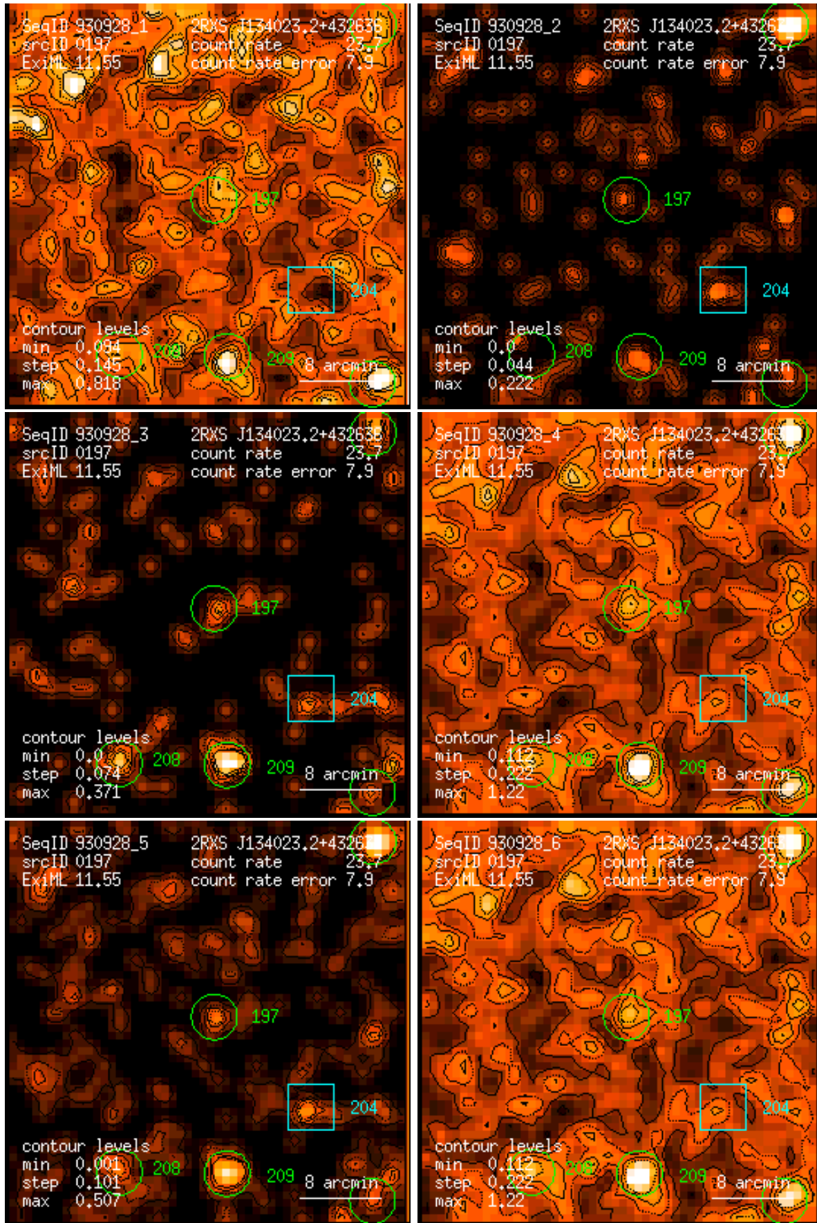
Figure 197: RASS 930928: detection 0197: band rate images, Gaussian filter: (1) PSPC channels 11 – 41, (2) 52 – 90, (3) 91 – 201, (4) 11 – 235, (5) 52 – 201, (6) 11 – 201. Broad band rates in counts/ks. Band rate contour levels in counts/ks/arcmin 2 .
