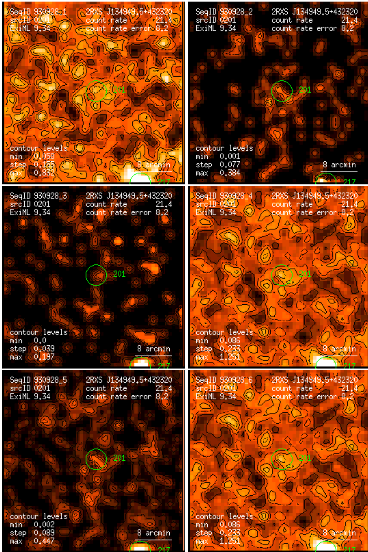
Figure 201: RASS 930928: detection 0201: band rate images, Gaussian filter: (1) PSPC channels 11 – 41, (2) 52 – 90, (3) 91 – 201, (4) 11 – 235, (5) 52 – 201, (6) 11 – 201. Broad band rates in counts/ks. Band rate contour levels in counts/ks/arcmin 2 .
