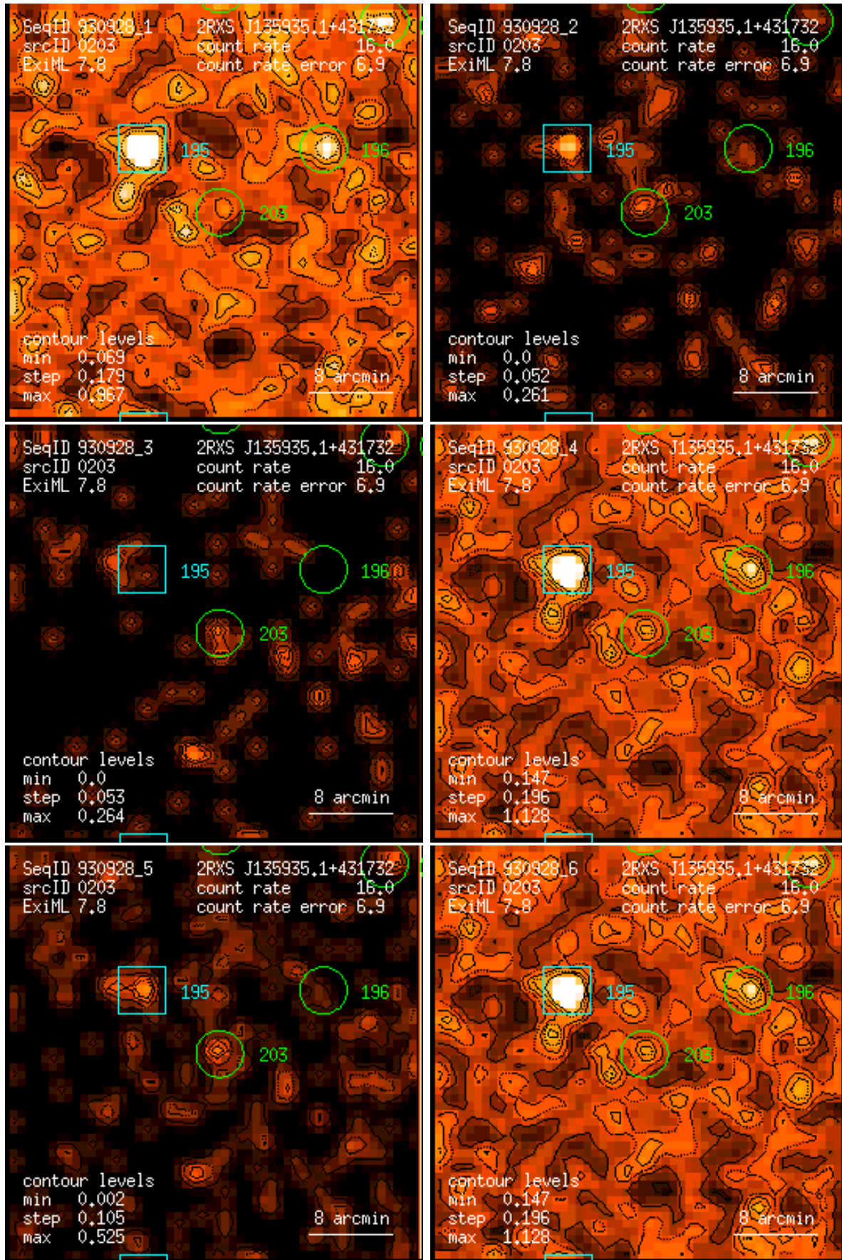
Figure 203: RASS 930928: detection 0203: band rate images, Gaussian filter: (1) PSPC channels 11 – 41, (2) 52 – 90, (3) 91 – 201, (4) 11 – 235, (5) 52 – 201, (6) 11 – 201. Broad band rates in counts/ks. Band rate contour levels in counts/ks/arcmin 2 .
