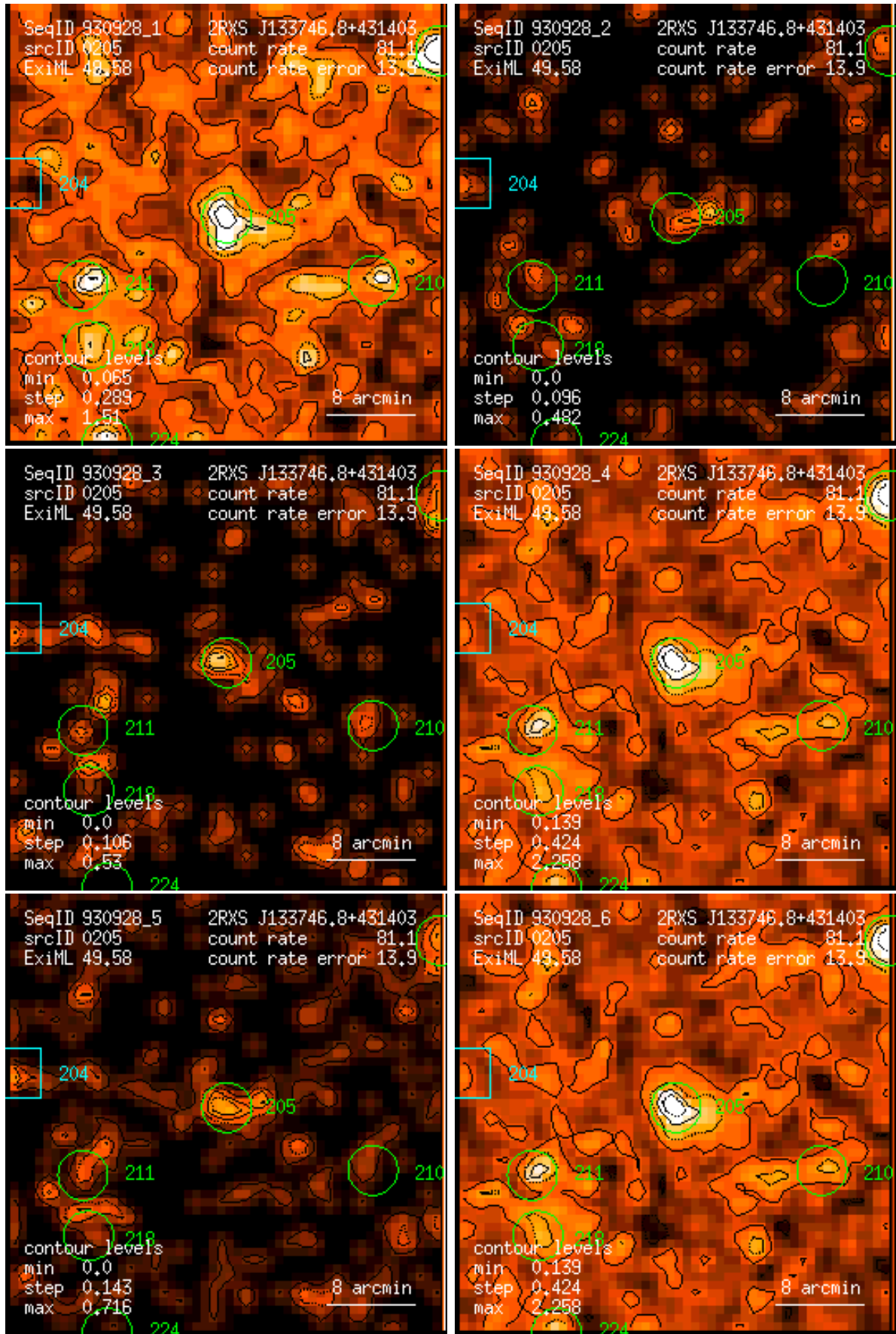
Figure 205: RASS 930928: detection 0205: band rate images, Gaussian filter: (1) PSPC channels 11 – 41, (2) 52 – 90, (3) 91 – 201, (4) 11 – 235, (5) 52 – 201, (6) 11 – 201. Broad band rates in counts/ks. Band rate contour levels in counts/ks/arcmin 2 .
