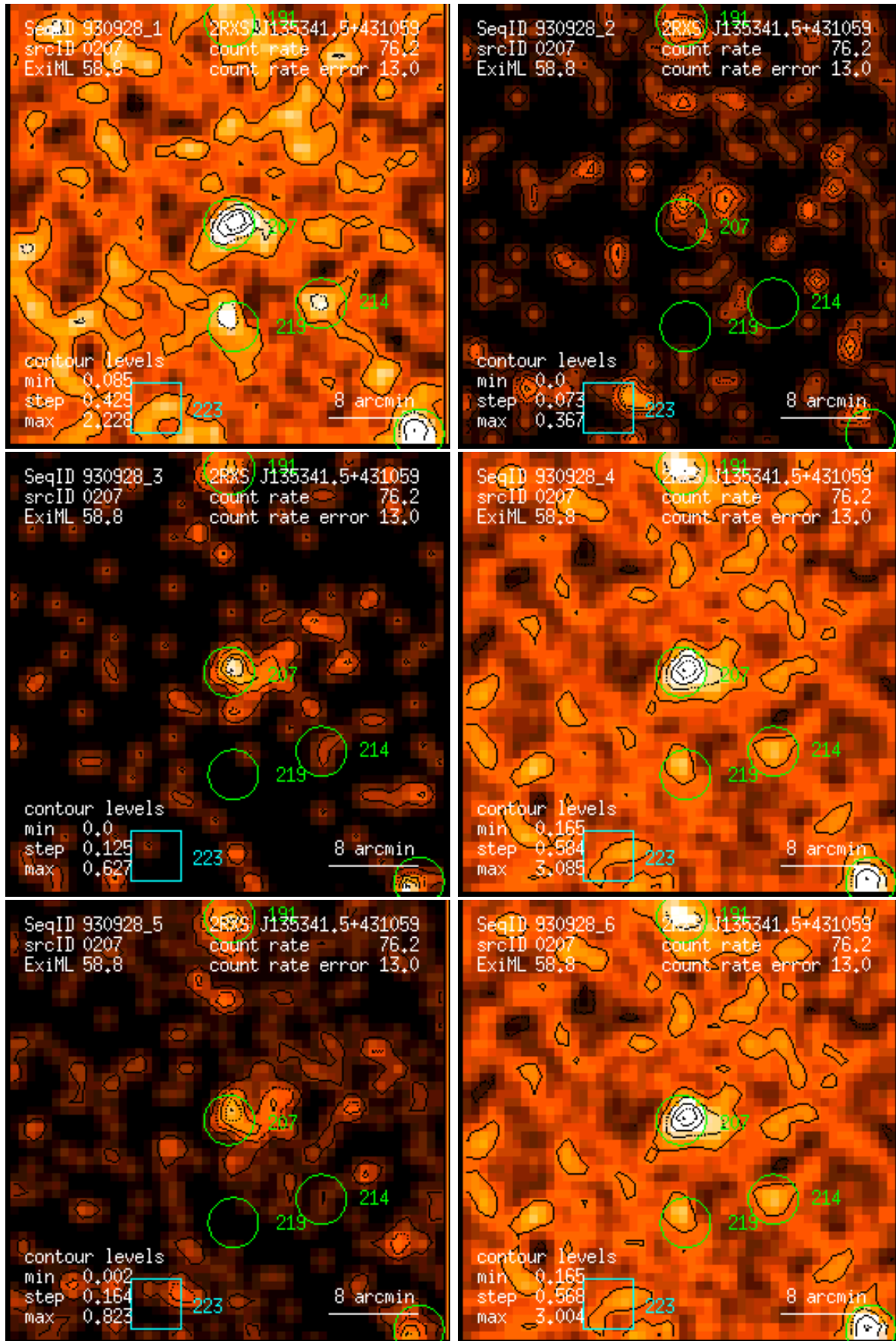
Figure 207: RASS 930928: detection 0207: band rate images, Gaussian filter: (1) PSPC channels 11 – 41, (2) 52 – 90, (3) 91 – 201, (4) 11 – 235, (5) 52 – 201, (6) 11 – 201. Broad band rates in counts/ks. Band rate contour levels in counts/ks/arcmin 2 .
