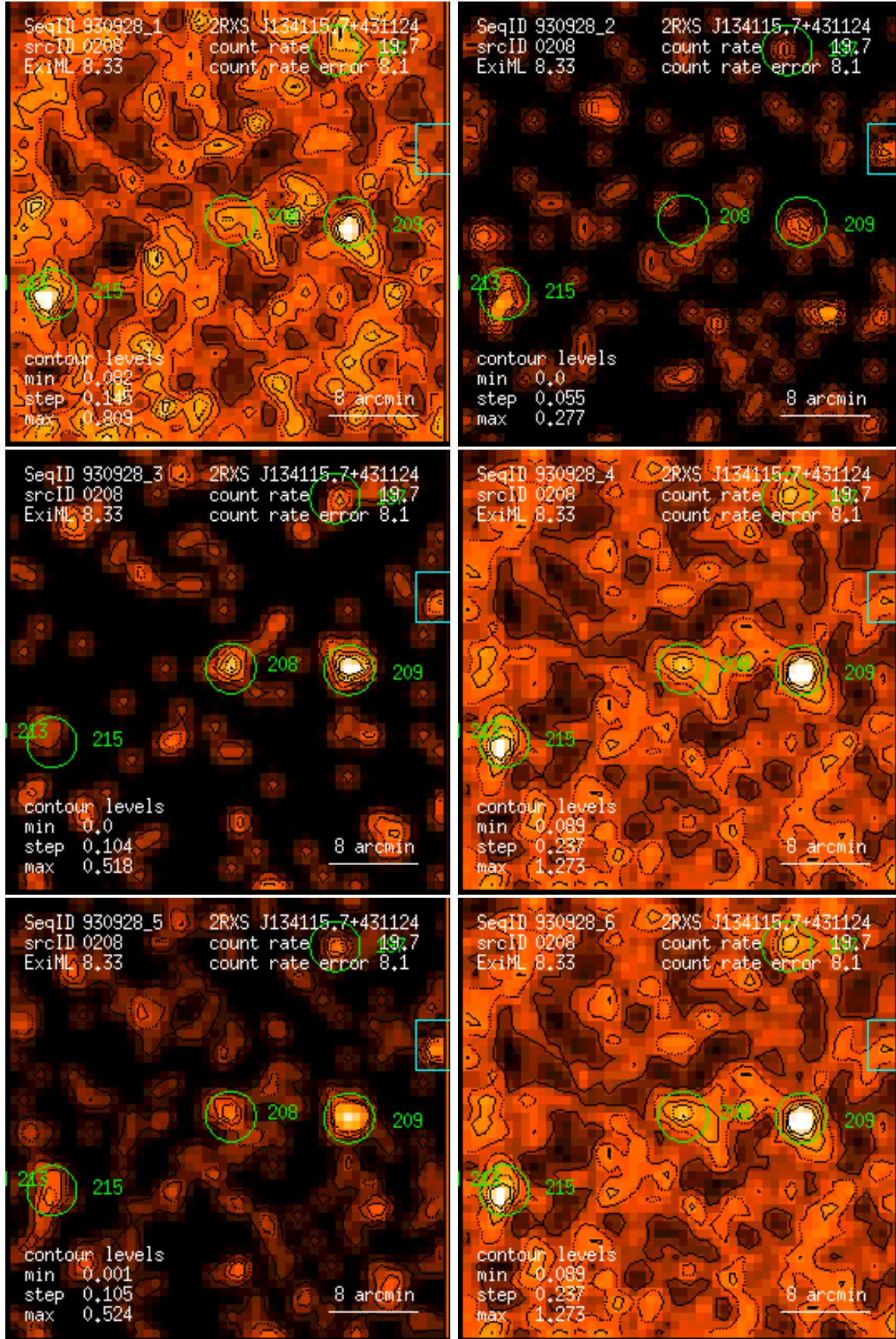
Figure 208: RASS 930928: detection 0208: band rate images, Gaussian filter: (1) PSPC channels 11 – 41, (2) 52 – 90, (3) 91 – 201, (4) 11 – 235, (5) 52 – 201, (6) 11 – 201. Broad band rates in counts/ks. Band rate contour levels in counts/ks/arcmin 2 .
