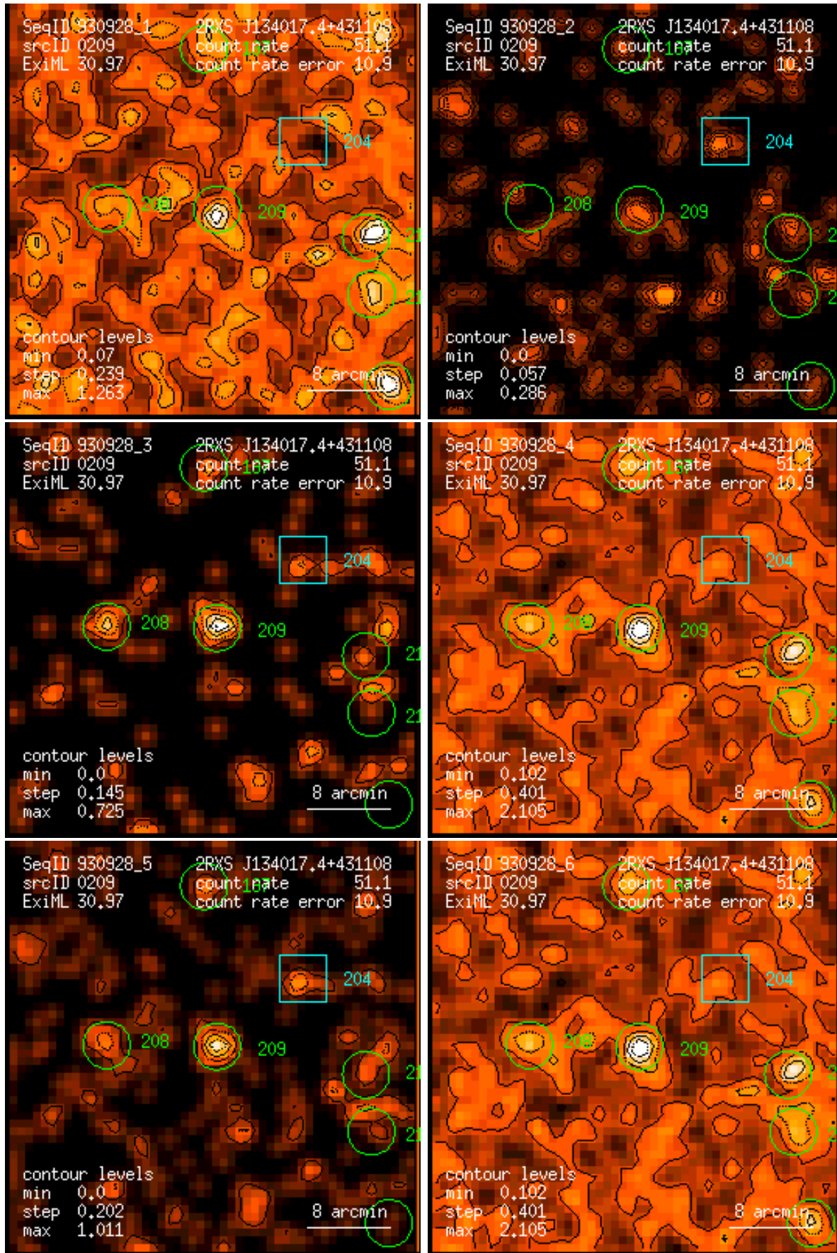
Figure 209: RASS 930928: detection 0209: band rate images, Gaussian filter: (1) PSPC channels 11 – 41, (2) 52 – 90, (3) 91 – 201, (4) 11 – 235, (5) 52 – 201, (6) 11 – 201. Broad band rates in counts/ks. Band rate contour levels in counts/ks/arcmin 2 .
