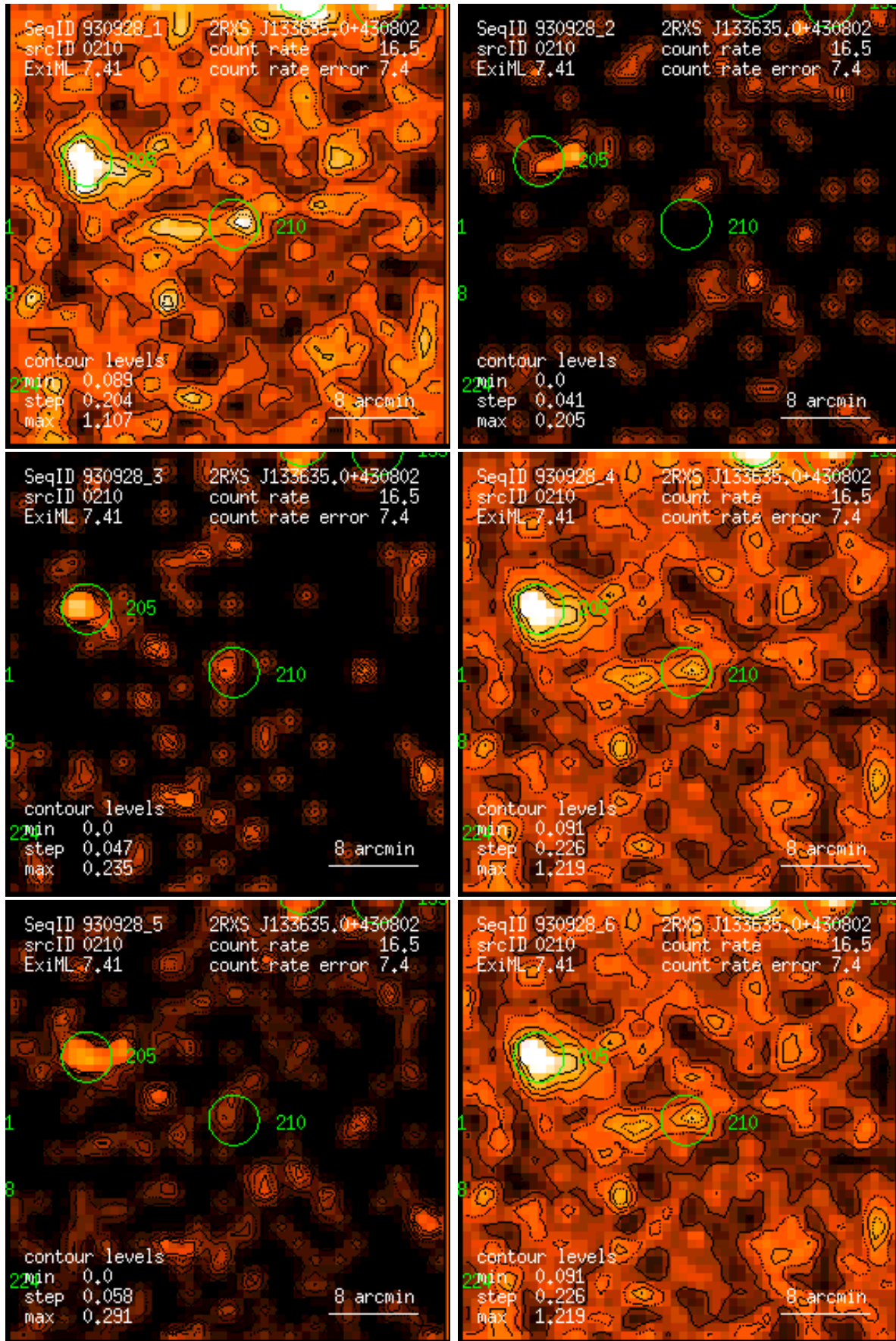
Figure 210: RASS 930928: detection 0210: band rate images, Gaussian filter: (1) PSPC channels 11 – 41, (2) 52 – 90, (3) 91 – 201, (4) 11 – 235, (5) 52 – 201, (6) 11 – 201. Broad band rates in counts/ks. Band rate contour levels in counts/ks/arcmin 2 .
