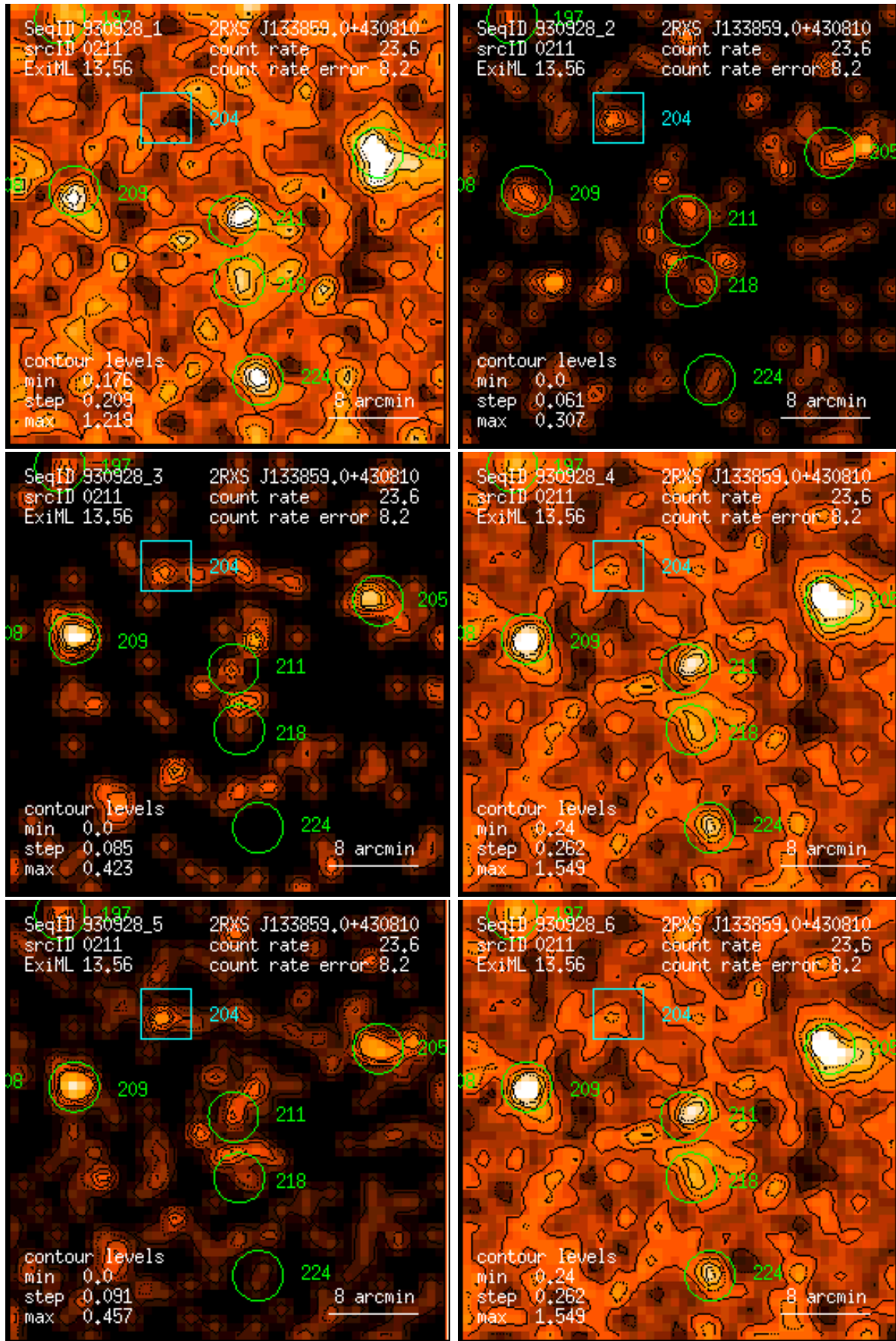
Figure 211: RASS 930928: detection 0211: band rate images, Gaussian filter: (1) PSPC channels 11 – 41, (2) 52 – 90, (3) 91 – 201, (4) 11 – 235, (5) 52 – 201, (6) 11 – 201. Broad band rates in counts/ks. Band rate contour levels in counts/ks/arcmin 2 .
