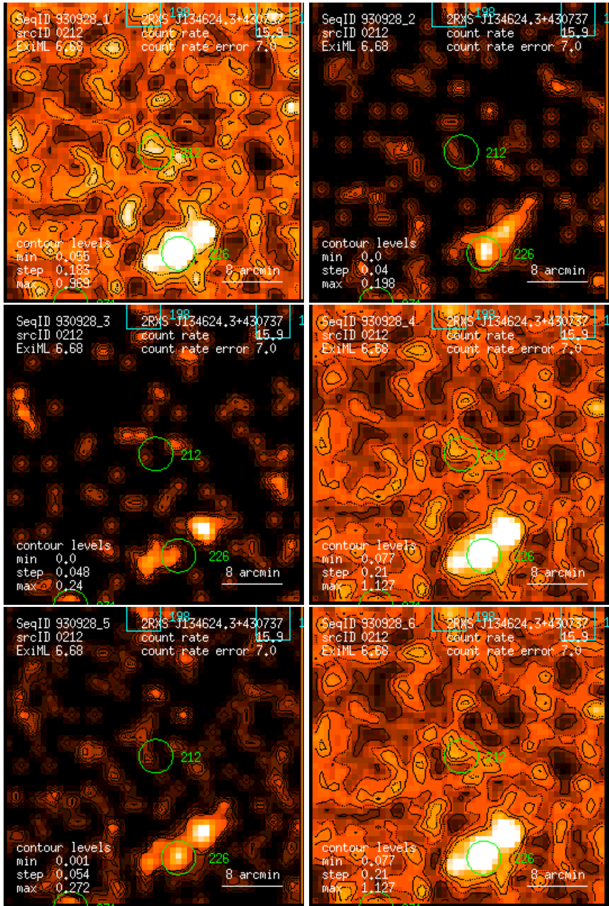
Figure 212: RASS 930928: detection 0212: band rate images, Gaussian filter: (1) PSPC channels 11 – 41, (2) 52 – 90, (3) 91 – 201, (4) 11 – 235, (5) 52 – 201, (6) 11 – 201. Broad band rates in counts/ks. Band rate contour levels in counts/ks/arcmin 2 .
