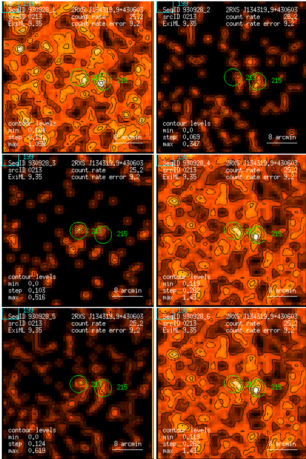
Figure 213: RASS 930928: detection 0213: band rate images, Gaussian filter: (1) PSPC channels 11 – 41, (2) 52 – 90, (3) 91 – 201, (4) 11 – 235, (5) 52 – 201, (6) 11 – 201. Broad band rates in counts/ks. Band rate contour levels in counts/ks/arcmin 2 .
