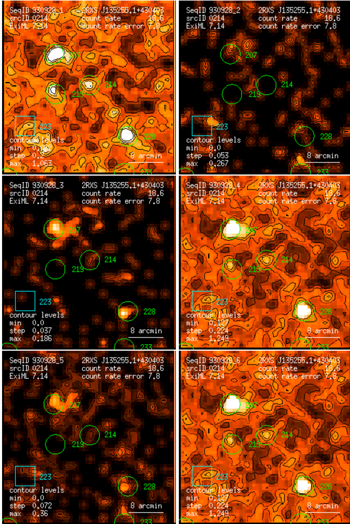
Figure 214: RASS 930928: detection 0214: band rate images, Gaussian filter: (1) PSPC channels 11 – 41, (2) 52 – 90, (3) 91 – 201, (4) 11 – 235, (5) 52 – 201, (6) 11 – 201. Broad band rates in counts/ks. Band rate contour levels in counts/ks/arcmin 2 .
