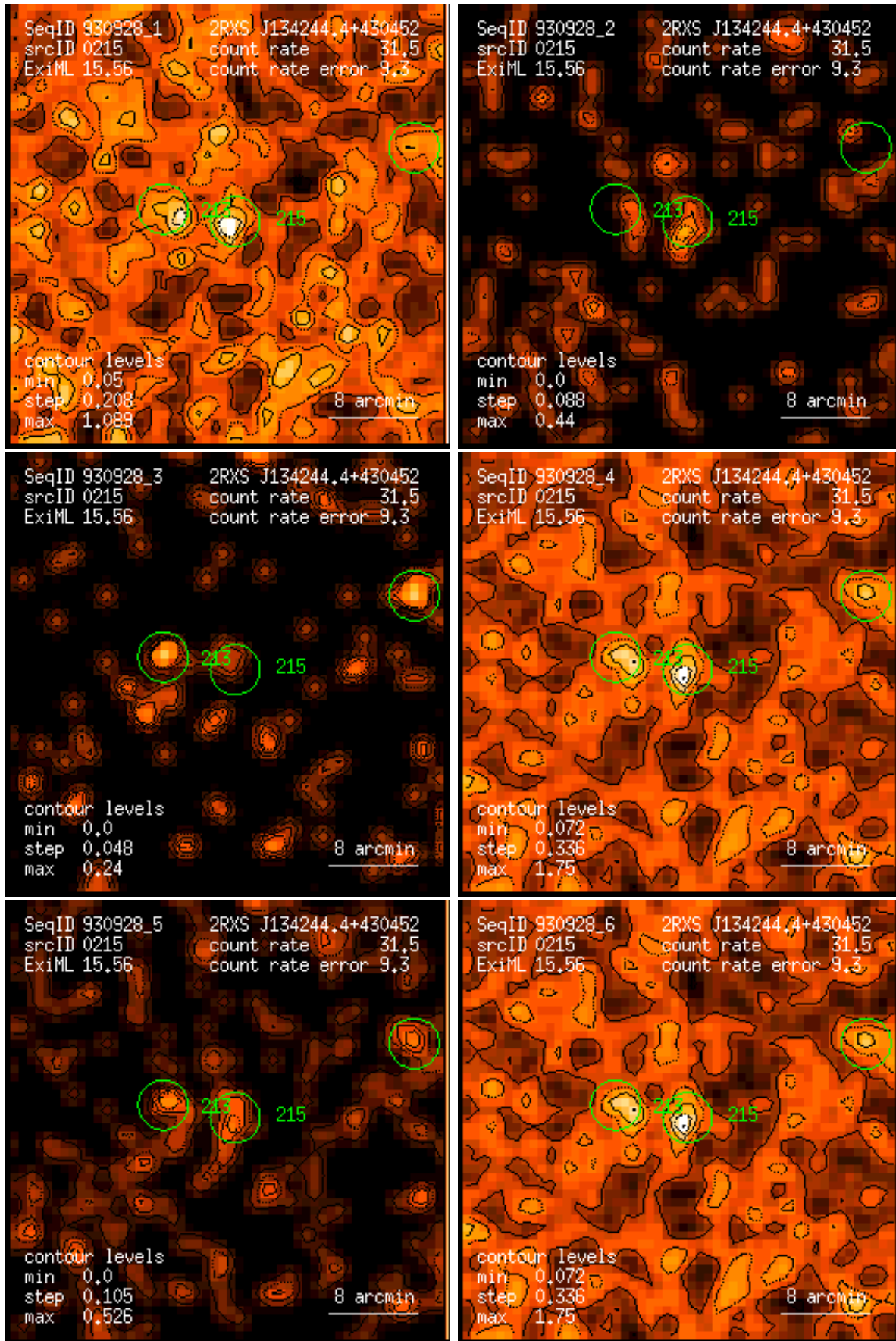
Figure 215: RASS 930928: detection 0215: band rate images, Gaussian filter: (1) PSPC channels 11 – 41, (2) 52 – 90, (3) 91 – 201, (4) 11 – 235, (5) 52 – 201, (6) 11 – 201. Broad band rates in counts/ks. Band rate contour levels in counts/ks/arcmin 2 .
