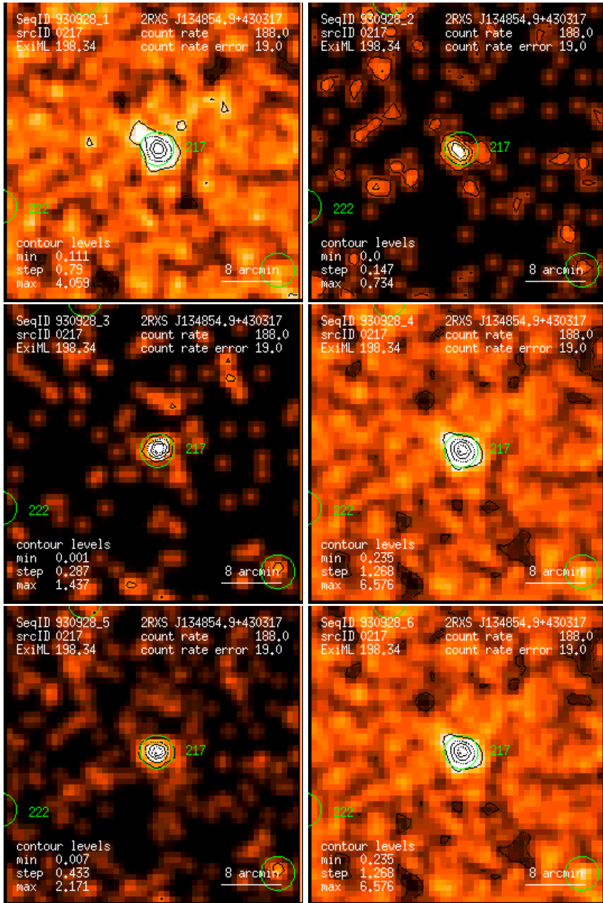
Figure 217: RASS 930928: detection 0217: band rate images, Gaussian filter: (1) PSPC channels 11 – 41, (2) 52 – 90, (3) 91 – 201, (4) 11 – 235, (5) 52 – 201, (6) 11 – 201. Broad band rates in counts/ks. Band rate contour levels in counts/ks/arcmin 2 .
