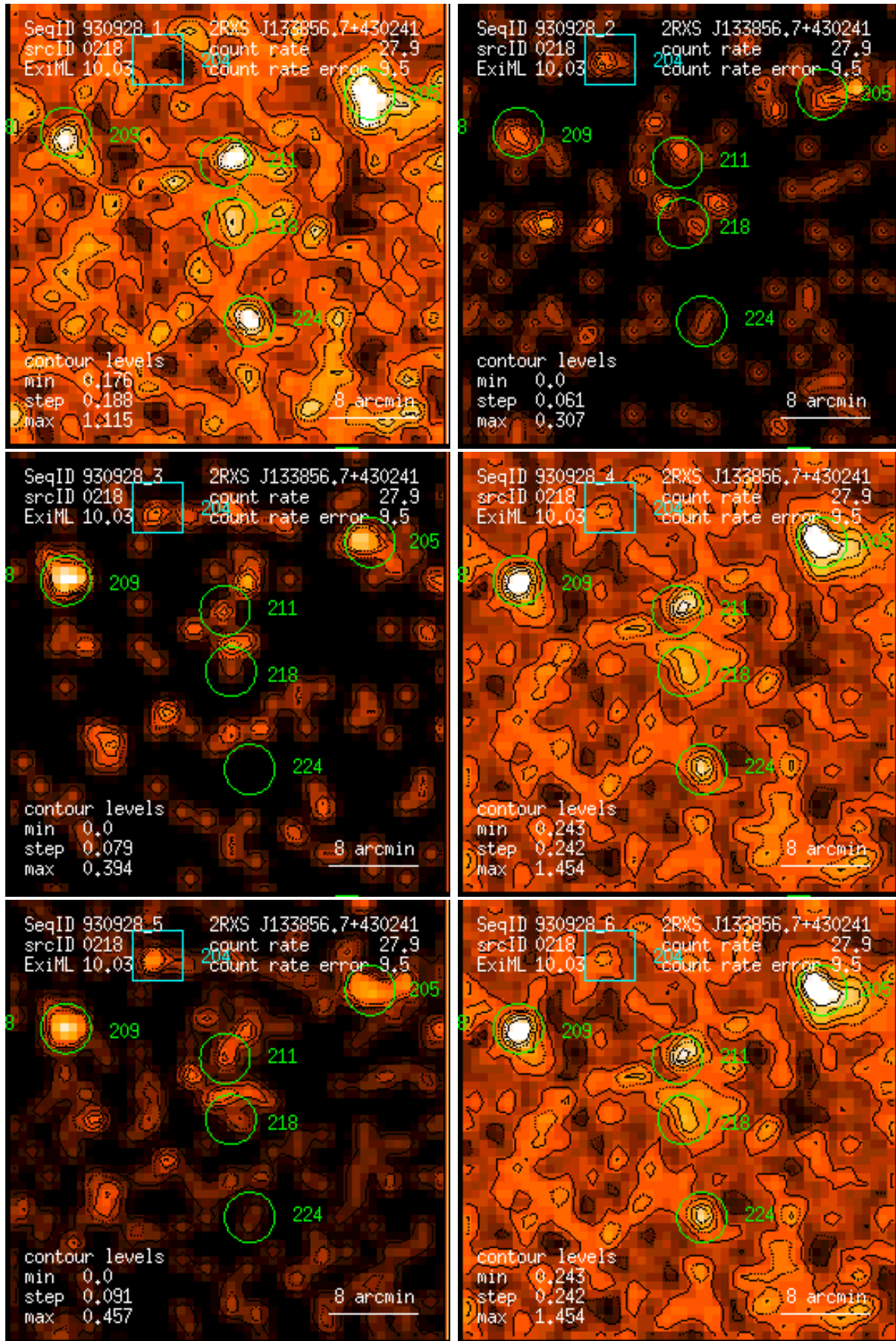
Figure 218: RASS 930928: detection 0218: band rate images, Gaussian filter: (1) PSPC channels 11 – 41, (2) 52 – 90, (3) 91 – 201, (4) 11 – 235, (5) 52 – 201, (6) 11 – 201. Broad band rates in counts/ks. Band rate contour levels in counts/ks/arcmin 2 .
