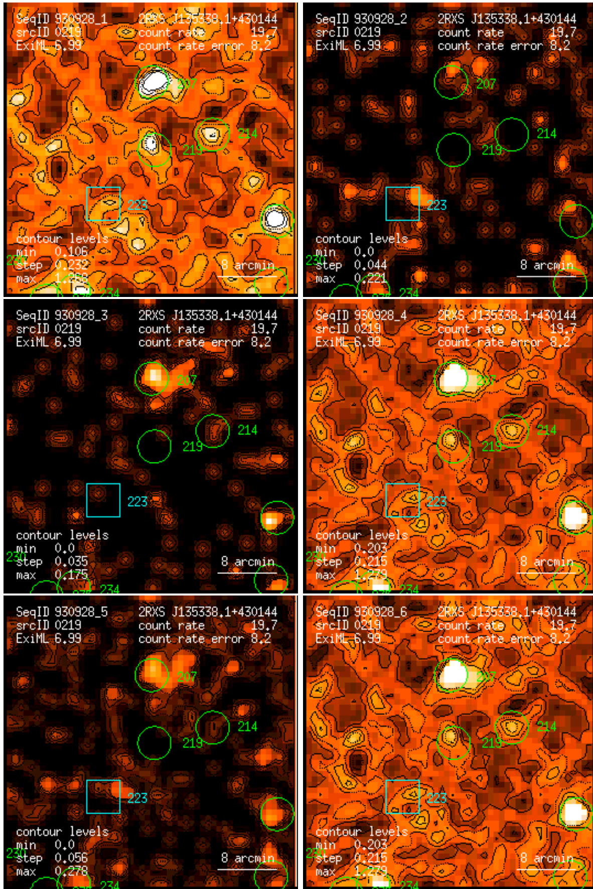
Figure 219: RASS 930928: detection 0219: band rate images, Gaussian filter: (1) PSPC channels 11 – 41, (2) 52 – 90, (3) 91 – 201, (4) 11 – 235, (5) 52 – 201, (6) 11 – 201. Broad band rates in counts/ks. Band rate contour levels in counts/ks/arcmin 2 .
