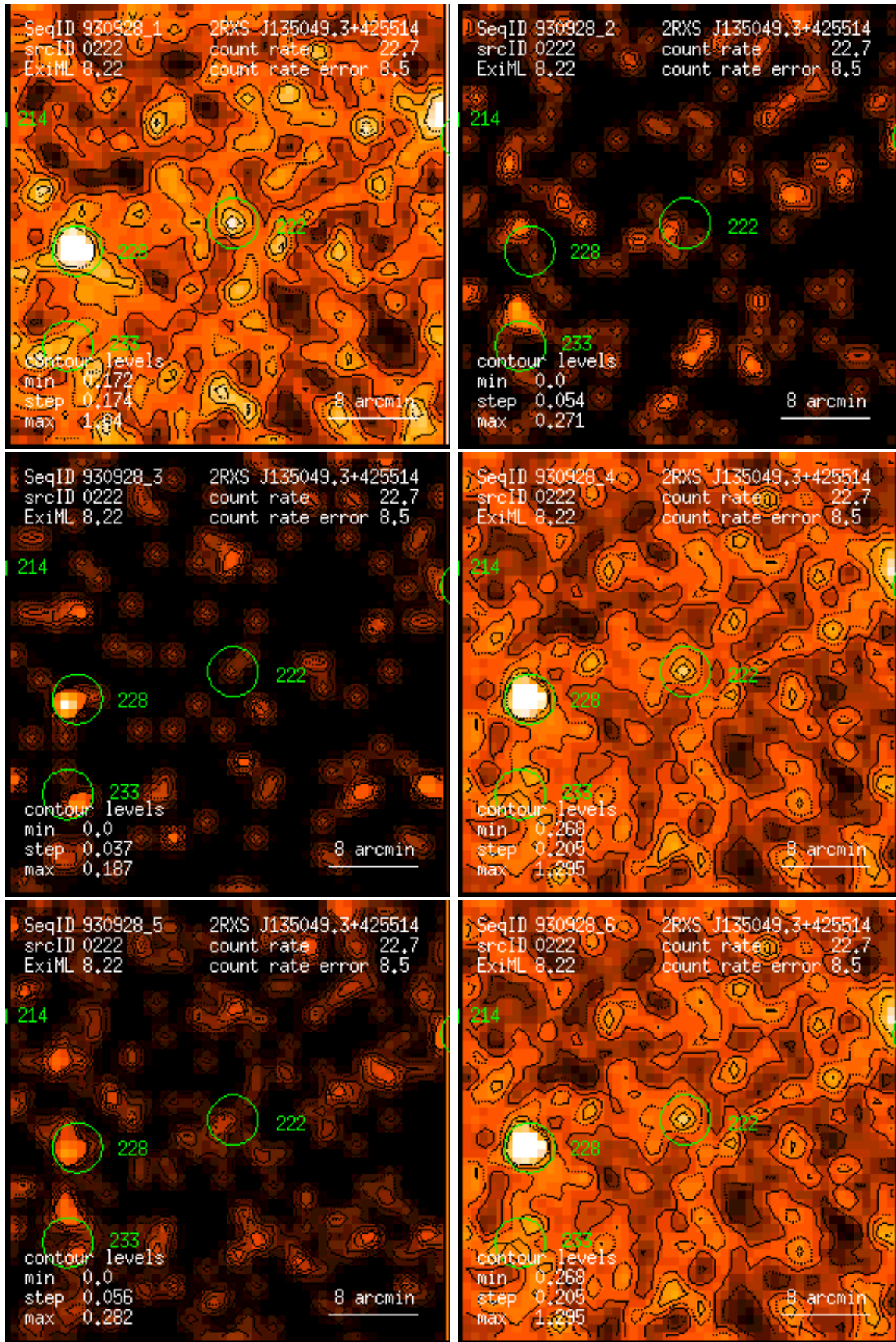
Figure 222: RASS 930928: detection 0222: band rate images, Gaussian filter: (1) PSPC channels 11 – 41, (2) 52 – 90, (3) 91 – 201, (4) 11 – 235, (5) 52 – 201, (6) 11 – 201. Broad band rates in counts/ks. Band rate contour levels in counts/ks/arcmin 2 .
