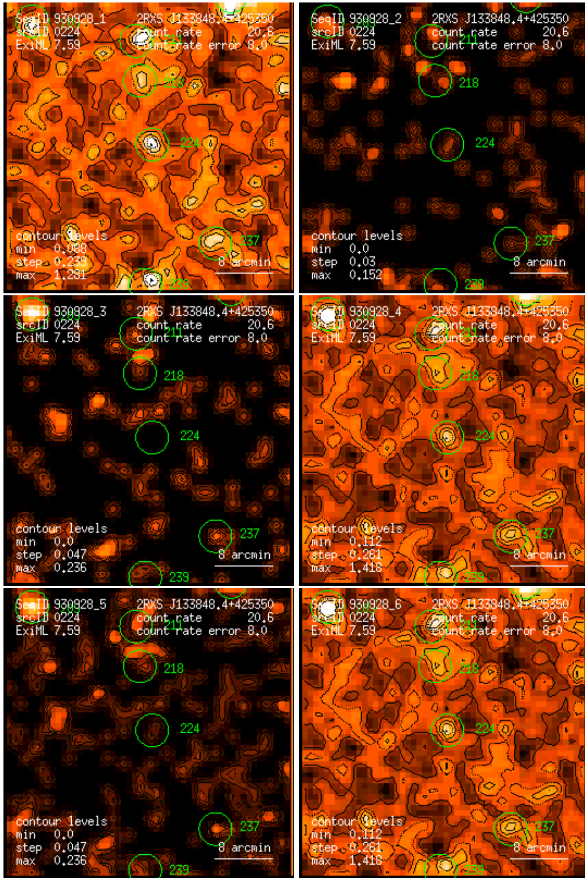
Figure 224: RASS 930928: detection 0224: band rate images, Gaussian filter: (1) PSPC channels 11 – 41, (2) 52 – 90, (3) 91 – 201, (4) 11 – 235, (5) 52 – 201, (6) 11 – 201. Broad band rates in counts/ks. Band rate contour levels in counts/ks/arcmin 2 .
