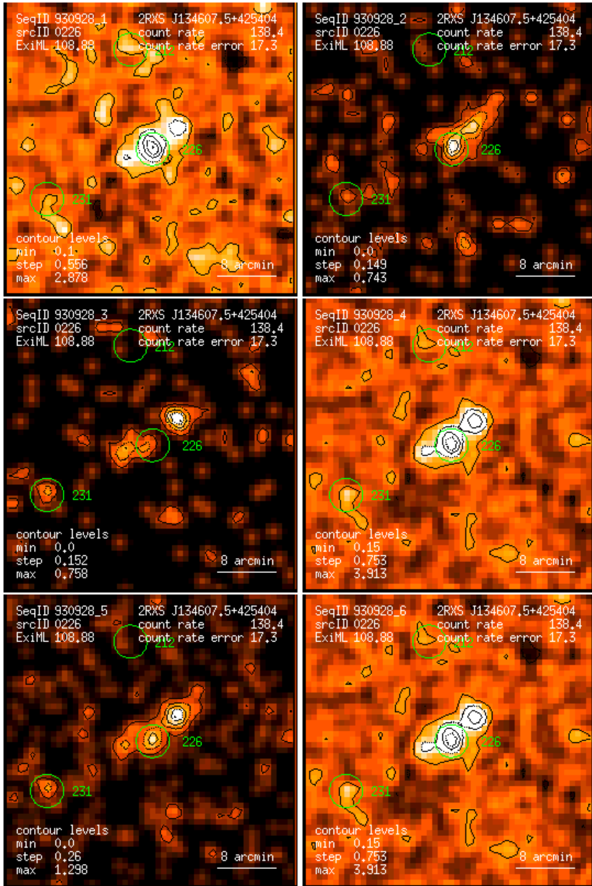
Figure 226: RASS 930928: detection 0226: band rate images, Gaussian filter: (1) PSPC channels 11 – 41, (2) 52 – 90, (3) 91 – 201, (4) 11 – 235, (5) 52 – 201, (6) 11 – 201. Broad band rates in counts/ks. Band rate contour levels in counts/ks/arcmin 2 .
