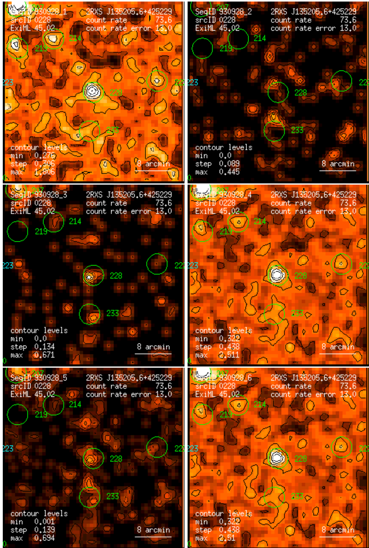
Figure 228: RASS 930928: detection 0228: band rate images, Gaussian filter: (1) PSPC channels 11 – 41, (2) 52 – 90, (3) 91 – 201, (4) 11 – 235, (5) 52 – 201, (6) 11 – 201. Broad band rates in counts/ks. Band rate contour levels in counts/ks/arcmin 2 .
