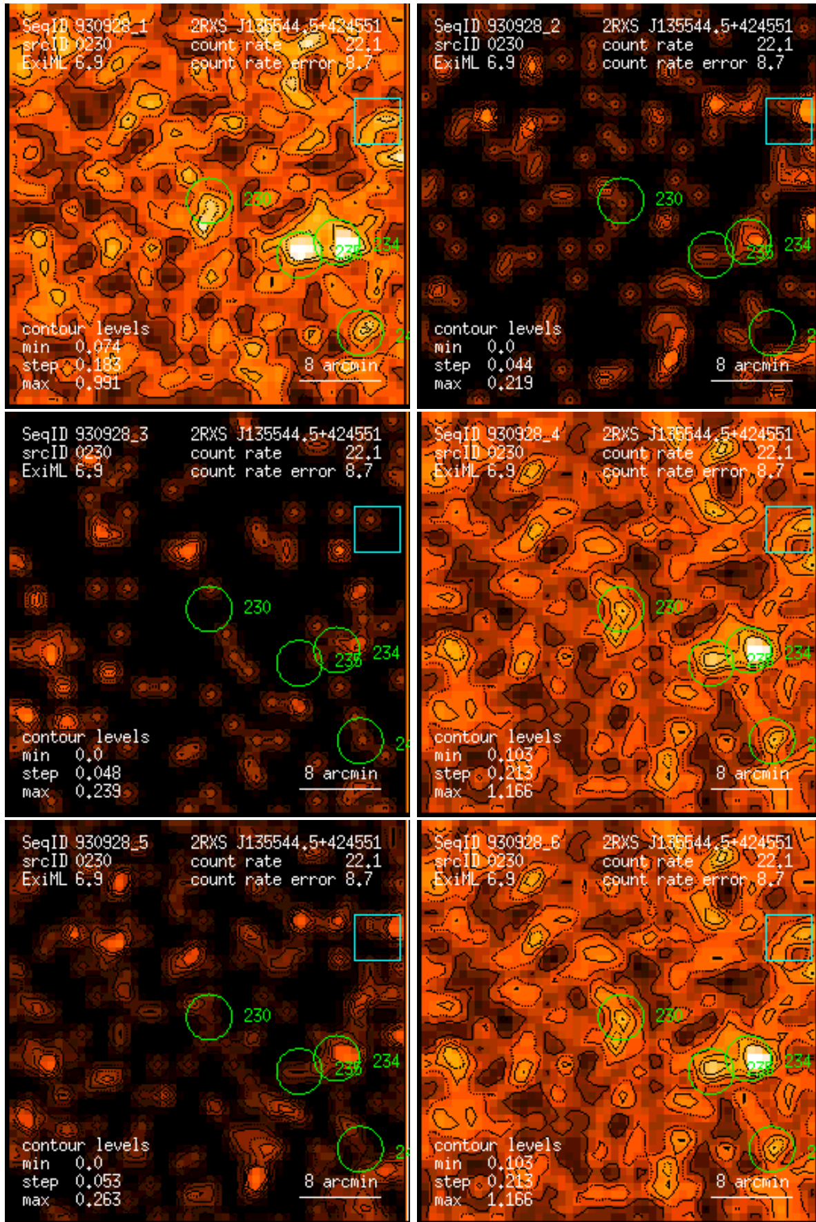
Figure 230: RASS 930928: detection 0230: band rate images, Gaussian filter: (1) PSPC channels 11 – 41, (2) 52 – 90, (3) 91 – 201, (4) 11 – 235, (5) 52 – 201, (6) 11 – 201. Broad band rates in counts/ks. Band rate contour levels in counts/ks/arcmin 2 .
