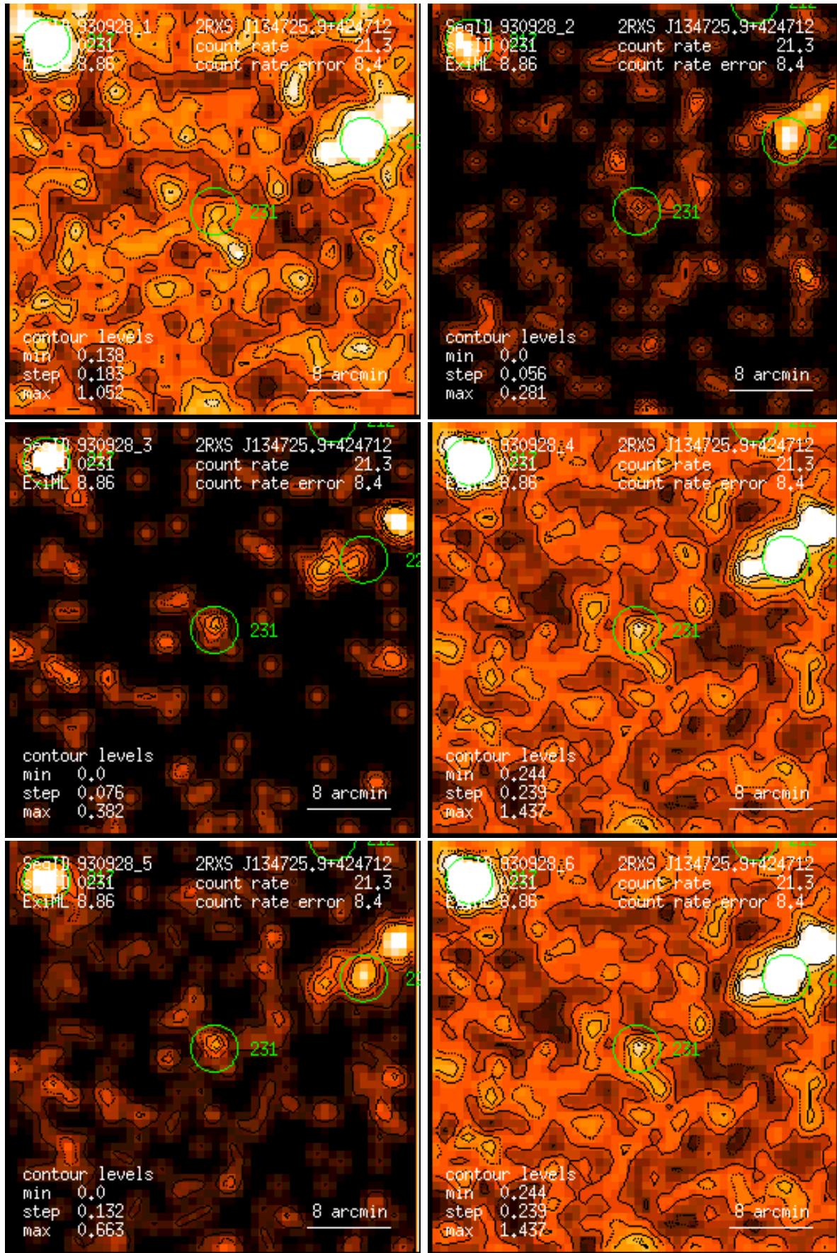
Figure 231: RASS 930928: detection 0231: band rate images, Gaussian filter: (1) PSPC channels 11 – 41, (2) 52 – 90, (3) 91 – 201, (4) 11 – 235, (5) 52 – 201, (6) 11 – 201. Broad band rates in counts/ks. Band rate contour levels in counts/ks/arcmin 2 .
