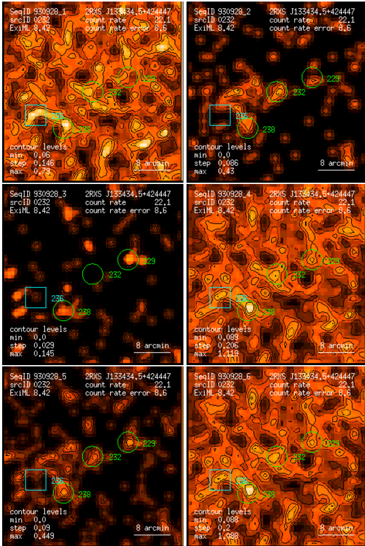
Figure 232: RASS 930928: detection 0232: band rate images, Gaussian filter: (1) PSPC channels 11 – 41, (2) 52 – 90, (3) 91 – 201, (4) 11 – 235, (5) 52 – 201, (6) 11 – 201. Broad band rates in counts/ks. Band rate contour levels in counts/ks/arcmin 2 .
