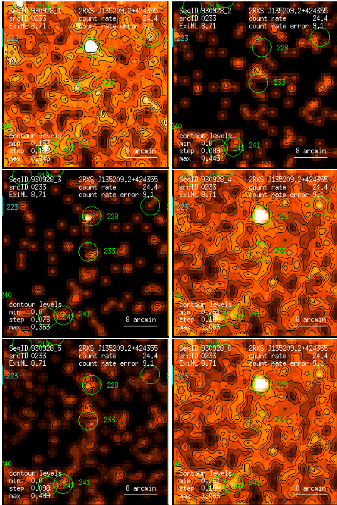
Figure 233: RASS 930928: detection 0233: band rate images, Gaussian filter: (1) PSPC channels 11 – 41, (2) 52 – 90, (3) 91 – 201, (4) 11 – 235, (5) 52 – 201, (6) 11 – 201. Broad band rates in counts/ks. Band rate contour levels in counts/ks/arcmin 2 .
