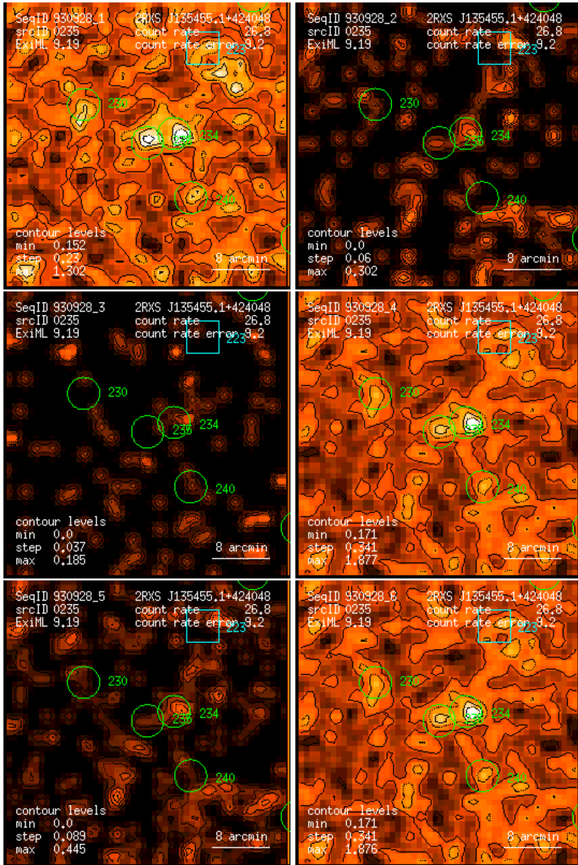
Figure 235: RASS 930928: detection 0235: band rate images, Gaussian filter: (1) PSPC channels 11 – 41, (2) 52 – 90, (3) 91 – 201, (4) 11 – 235, (5) 52 – 201, (6) 11 – 201. Broad band rates in counts/ks. Band rate contour levels in counts/ks/arcmin 2 .
