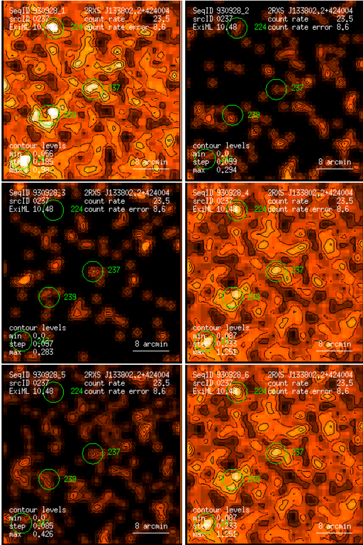
Figure 237: RASS 930928: detection 0237: band rate images, Gaussian filter: (1) PSPC channels 11 – 41, (2) 52 – 90, (3) 91 – 201, (4) 11 – 235, (5) 52 – 201, (6) 11 – 201. Broad band rates in counts/ks. Band rate contour levels in counts/ks/arcmin 2 .
